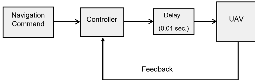
Fig. 9 Input delay diagram
