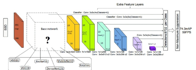
Figure 6. Single Shot Multibox Detector architecture. Extracted from [Jee et al., 2021].
