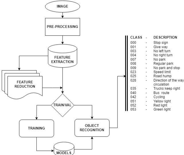
Figure 8. System overview. Adapted from [Alghmgham et al. , 2019].
