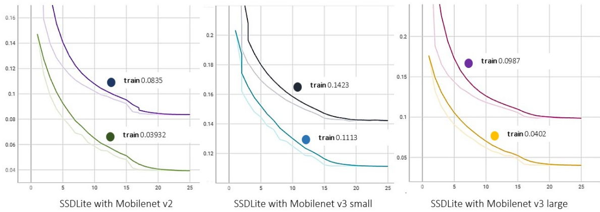
Figure 9. Loss for input size 320. Source: [Pierre and Fernandes, 2023].
