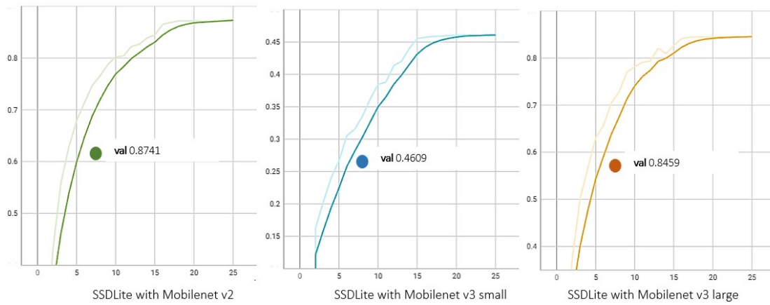
Figure 10. Accuracy for input size 320. Source: [Pierre and Fernandes, 2023].
