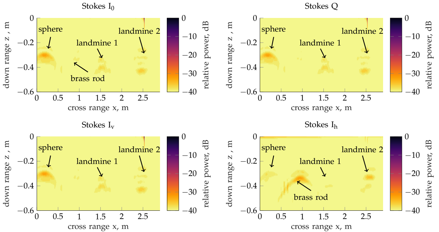
Figure 9: Top: Stokes parameters I_0 and Q , Bottom: I_v and I_h .
