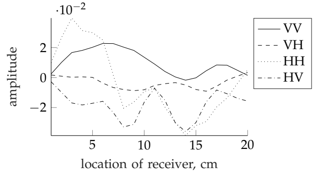
Figure 7: Difference in amplitude of 20 increments away from calibration target A_c .
