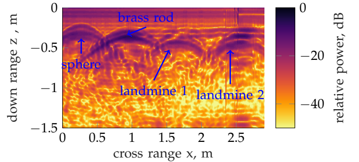
Figure 3: HH polarisation B-scan image of the radar scene with targets indicated.
