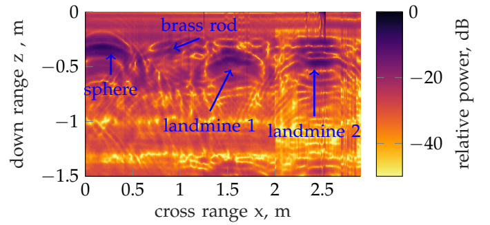
Figure 2: VV polarisation B-scan image of the radar scene with targets indicated.
