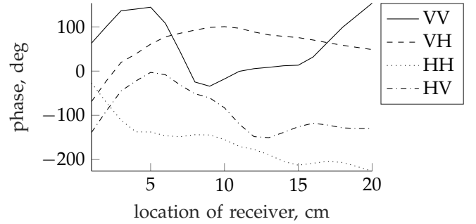
Figure 6: Difference in Phase of 20 increments away from calibration target \Phi_c .
