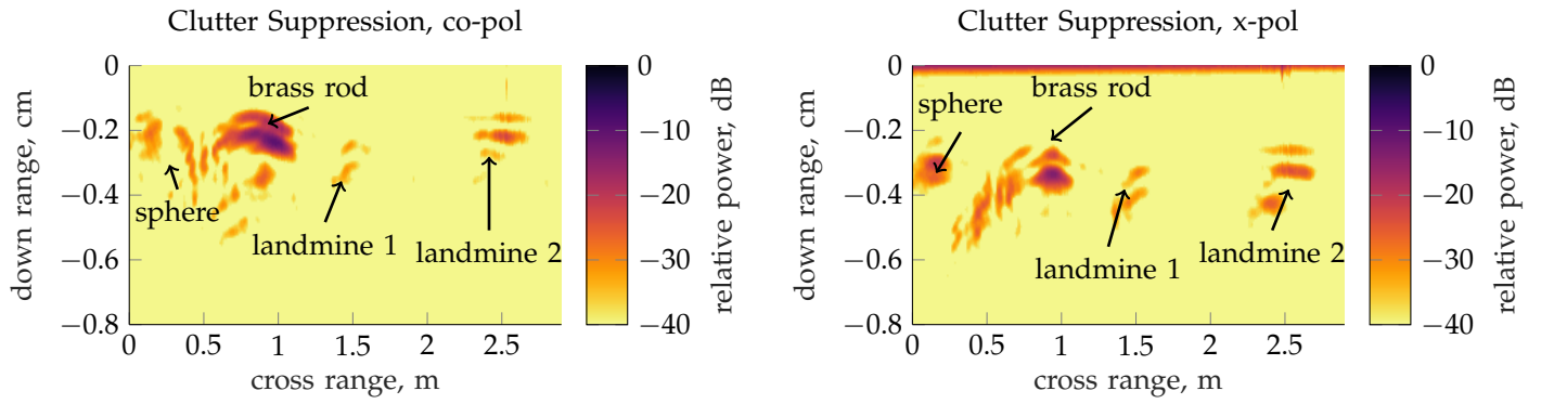
Figure 8: Co- and cross-polar polarimetric clutter suppression.
