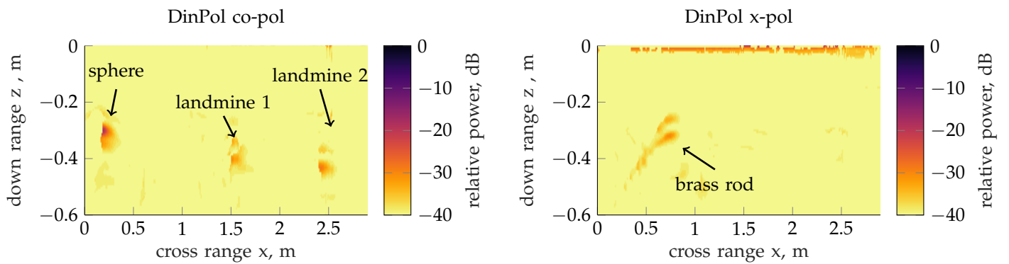
Figure 10: Co- and cross-polar DinPol results.
