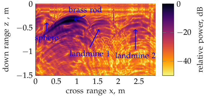
Figure 4: HV polarisation B-scan image of the radar scene with targets indicated.
