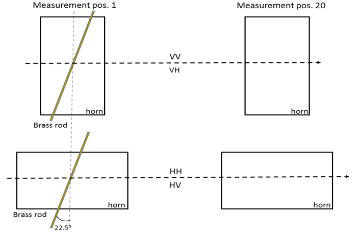
Figure 5: Schematic diagram illustrating the polarimetric correction calibration procedure.
