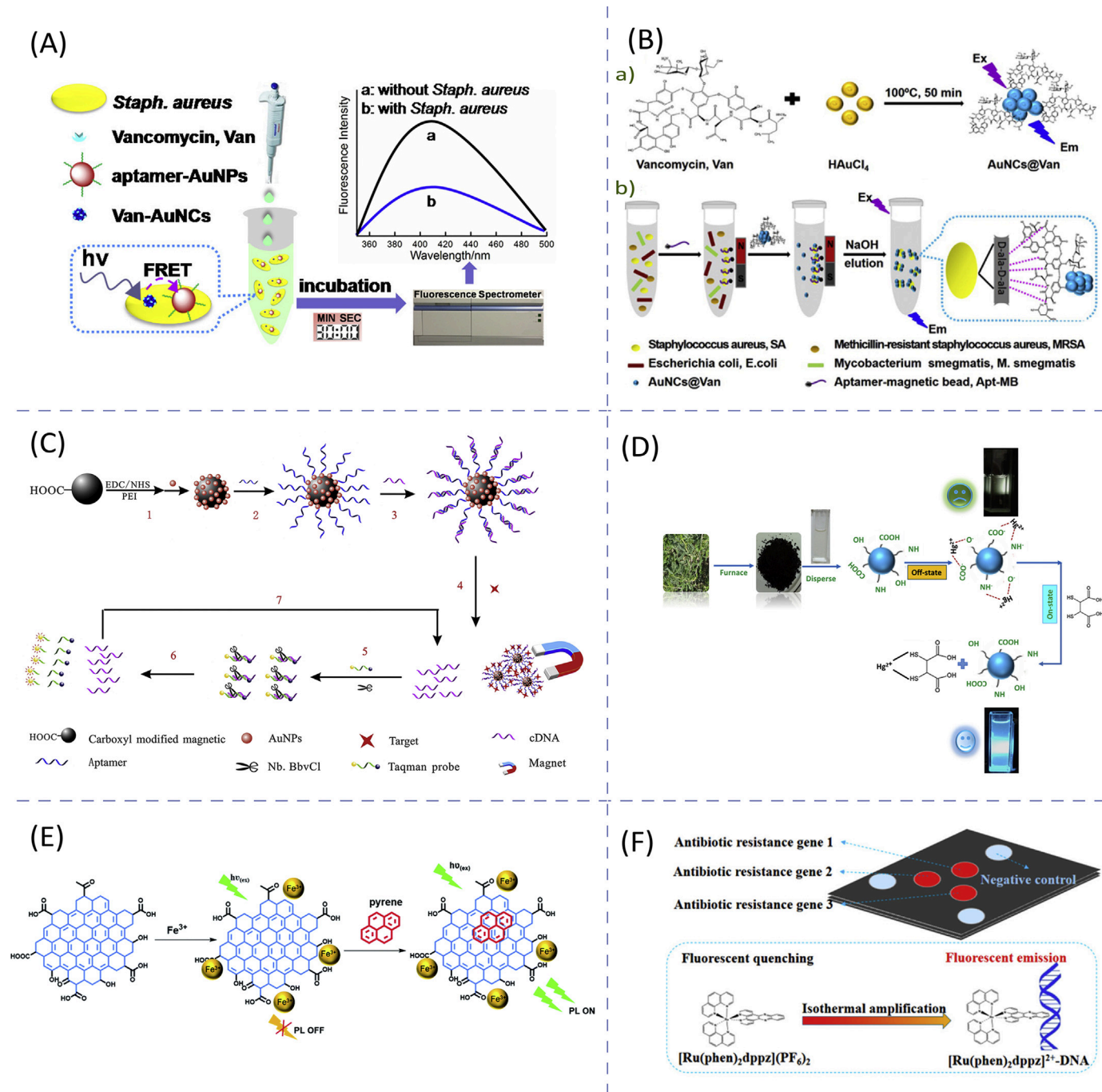
Fig. 2. (A) Schematic illustration of vancomycin based aptasensor for Staph. aureus [114]; (B) Schematic Illustrations of a) Preparation of AuNCs@Van, and b) Detection process for SA in using Apt-MB and AuNCs@Van [115]; (C) Schematic illustration for the detection of ampicillin amplified strategy for fluorescence signal using AuNPs/MBs with a nicking enzyme [116]; (D) Detection principle of turn-off/on fluorescence probe based on the green CQDs [117]; (E) Schematic illustration of the working mechanism of GQDs with Fe 3+ for fluorescence quenching and the turn-on mode with pyrene [118]; (F) Schematic illustration of the interaction of different ARGs [119].
