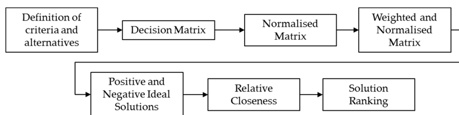
Figure 1. TOPSIS methodology.
