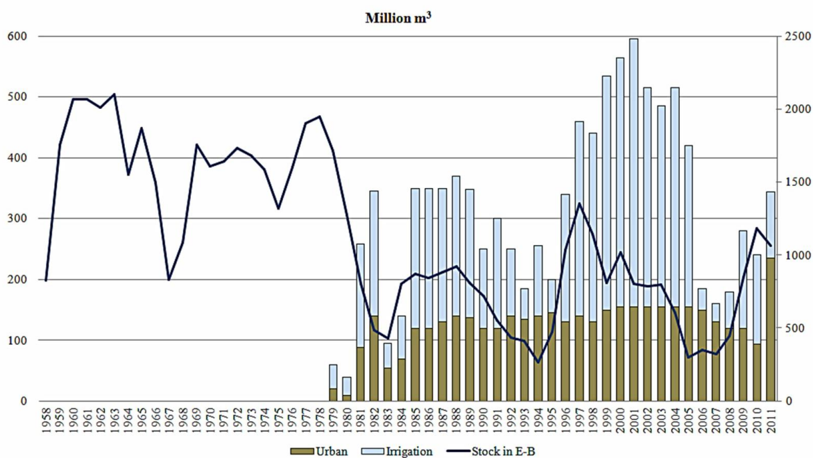
Fig. 2 Annual stored volume in Entrepeñas-Buendía (blue line, right axis) and volumes transferred for irrigators and urban suppliers through the Tagus-Segura Transfer, 1979-2011(million m 3 , left axis). Source: (CHT 2011) and San Martín (2011)
