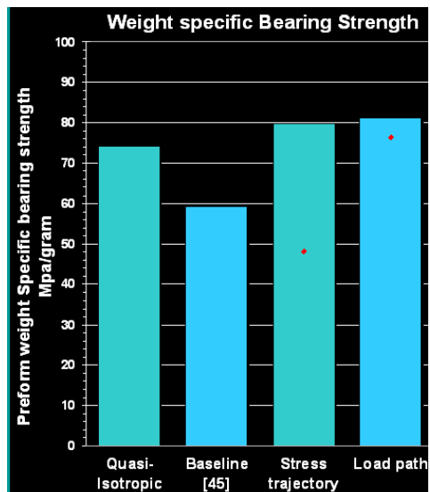
Figure 11. Weight specific bearing strength results
