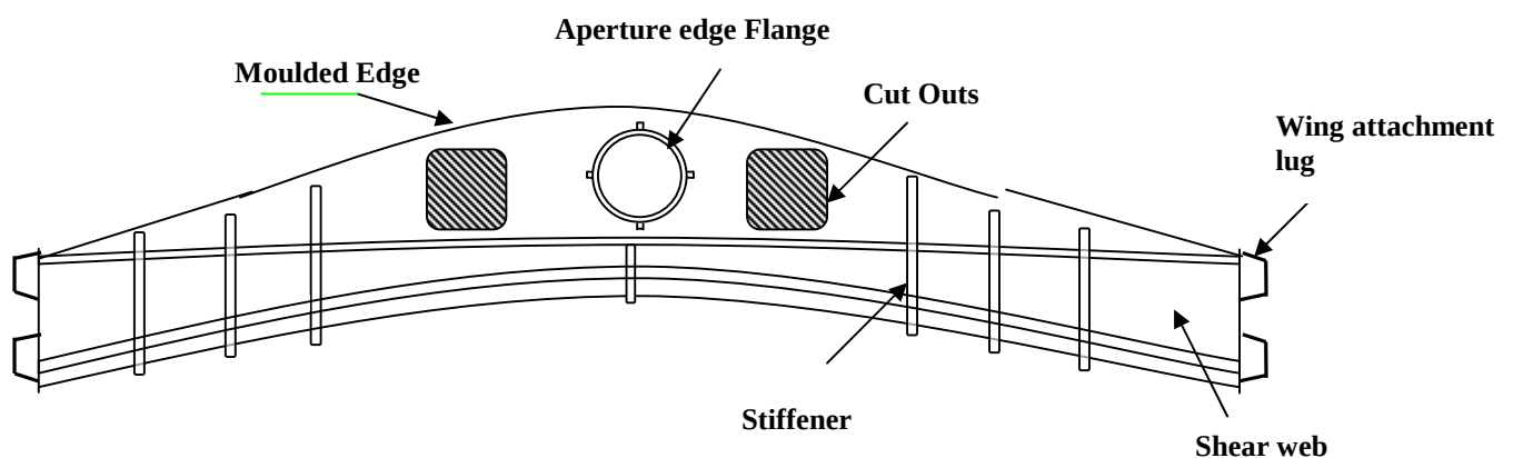
Figure 2. Generic carbon fibre composite spar design scheme
