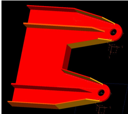
Figure 5. Frame shear web and attachment lug – 1 st stage design
