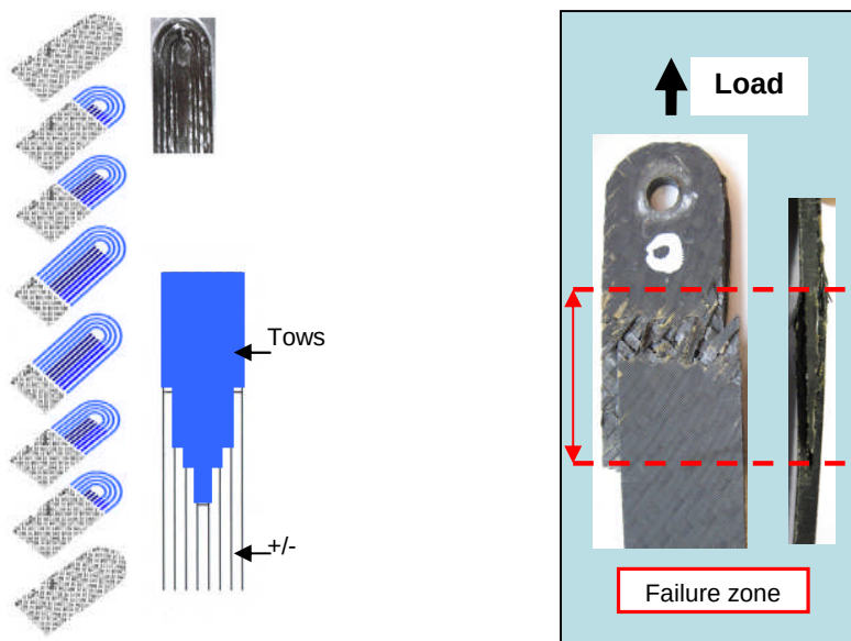
Figure 12. Arranged tow design with 6 fabric layers replaced
