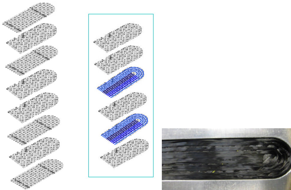
Figure 9. Baseline fabric lay up and example of arranged tow lay up.
