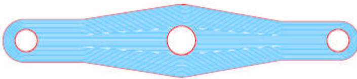
Figure 4. Optimisation of roving for a connection beam for the tension load case. (from Temmen et al Ref. 1.)
