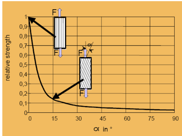
Figure 3. Variation in laminate strength with the angle of applied load
