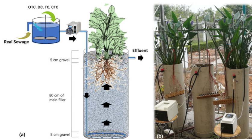
Figure 1. Schematic diagram of each system (a) and the photo of the experimental setup (b).
