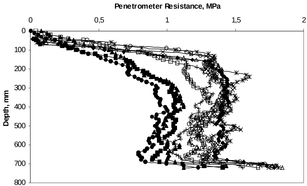
Fig. 7. Penetrometer resistance across the soil bin for the 900mm/10.5t/1.9bar tyre with ten readings: •, 1; ■, 2; +, 3; ▲, 4; ×, 5; ◆, 6; *, 7; ○, 8; □, 9; and ▲, 10
