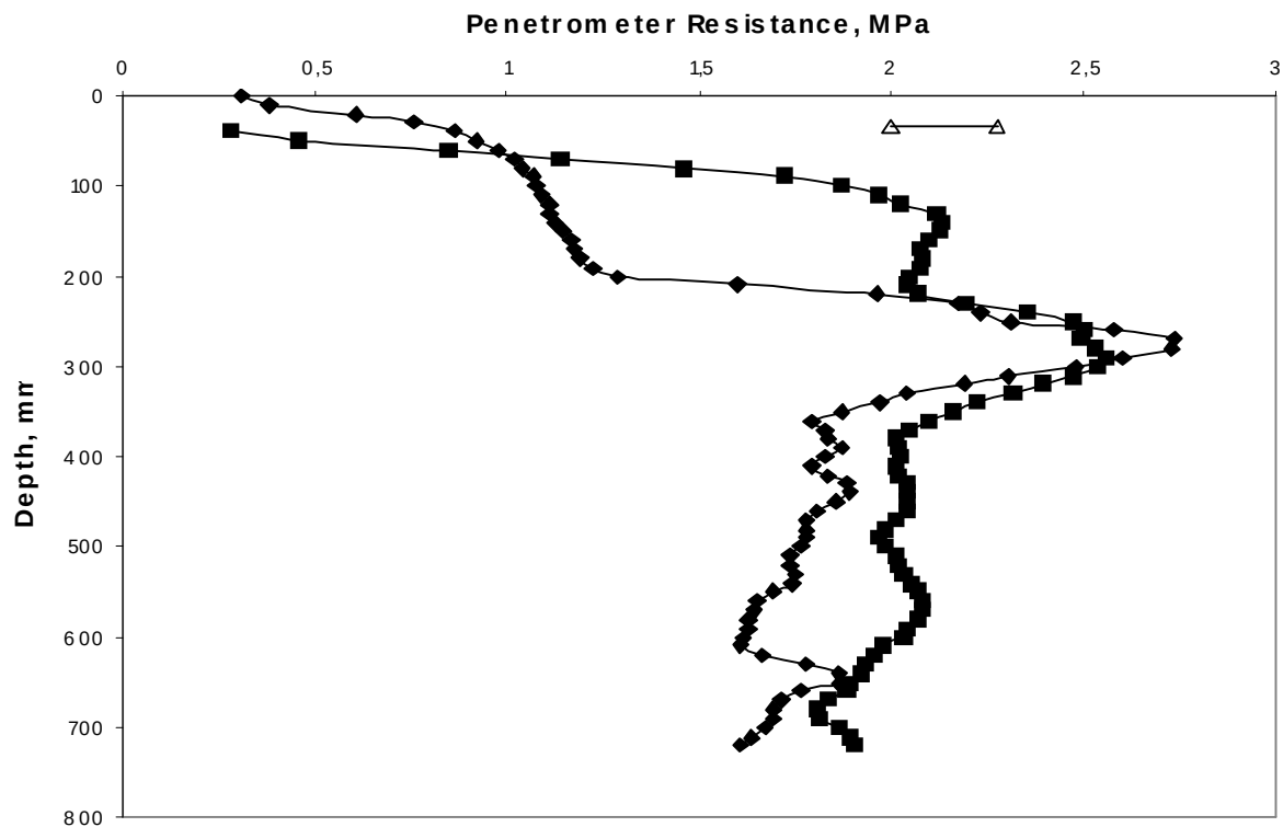
Fig. 15 a. Stratified soil conditions for the 900mm/10.5t/1.9bar: initial, \blacklozenge , and final, \blacksquare , including a least significant difference, \Delta , at 95% confidence level
