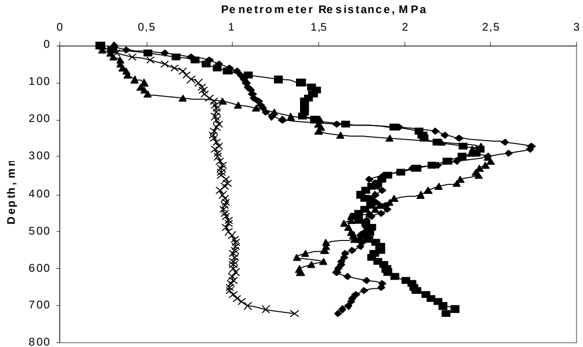
Fig. 2. Initial penetrometer resistance profiles in the soil bin of uniform and stratified soil conditions and including a field condition: ×, uniform; ■, ◆, stratified one and two; ▲, field condition
