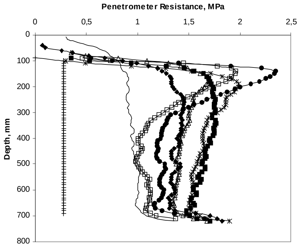
Fig. 11. Penetration resistance vs. depth initial and after the pass of the front tyres and the track: - , initial; *, 680mm/10.5t/2.2bar; ■, 800mm/10.5t/2.5bar; ◆, 900mm/10.5t/1.9bar; Δ, 800mm/10.5t/1.25bar; □, T10.5t; ●, T12t; and +, least significant difference at 95% confidence level
