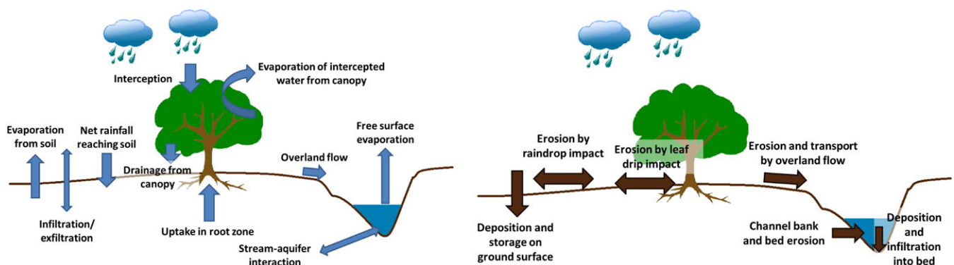
Figure 1. Hydrological and sediment erosion and deposition processes represented within the SHETRAN model. [Colour figure can be viewed at wileyonlinelibrary.com ]
