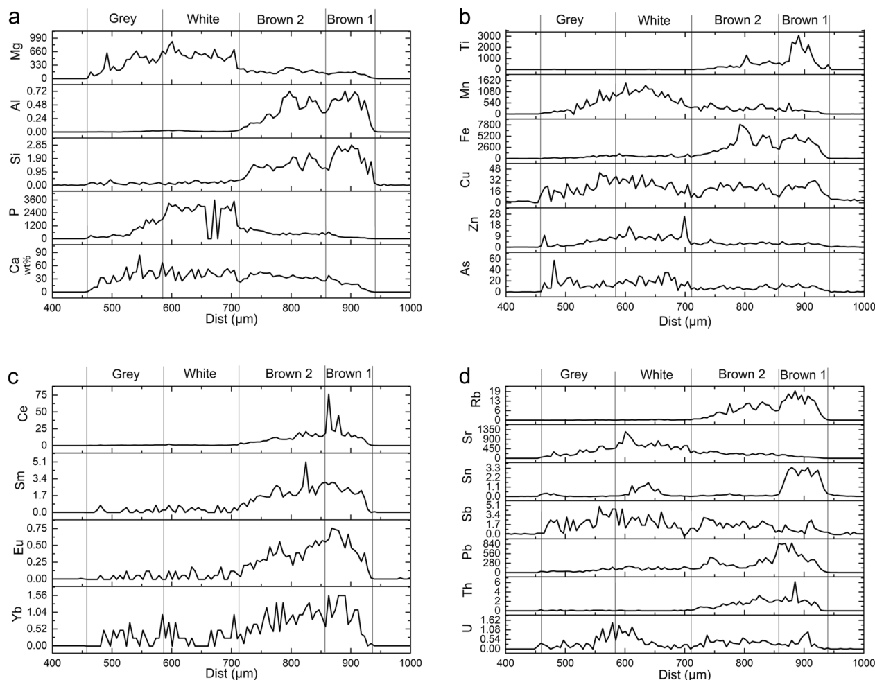
Fig. 6 a, b, c, and d: Calibrated LA-ICP-MS elemental concentrations in a 10 µm wide line perpendicular to the surface of sample KLR-2369/P2. Calcium is shown in wt%, while the rest is given in µg g -1
