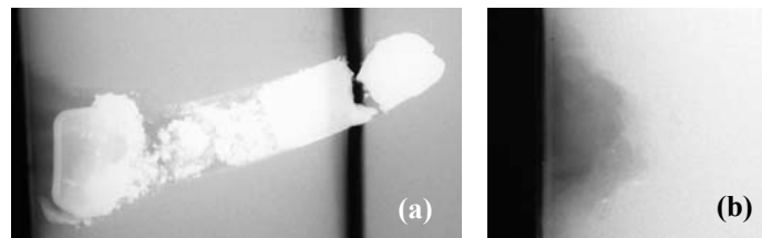
Figure 6: X-ray of the depth of penetration into the aluminium alloy witness block after completely penetrating (a) 5.48mm and (b) 6.52mm of Ceradyne silicon carbide (Ceralloy® 146-3E).
