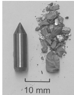
Figure 4: FFV core before and after perforating 5.44mm of Ceradyne silicon carbide (65% recovered mass).
