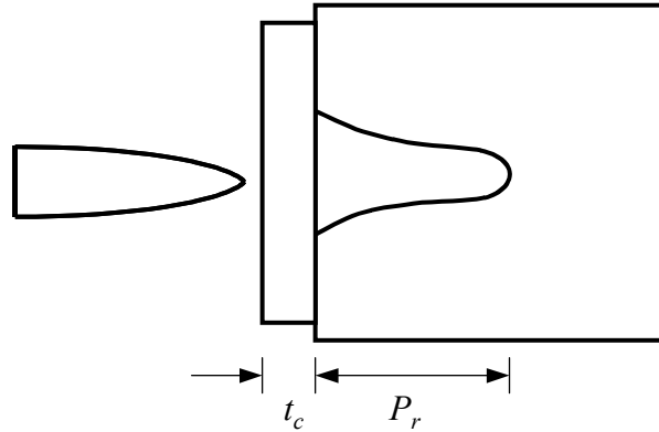
Figure 1: DOP technique for assessing each ceramic's ballistic performance.
