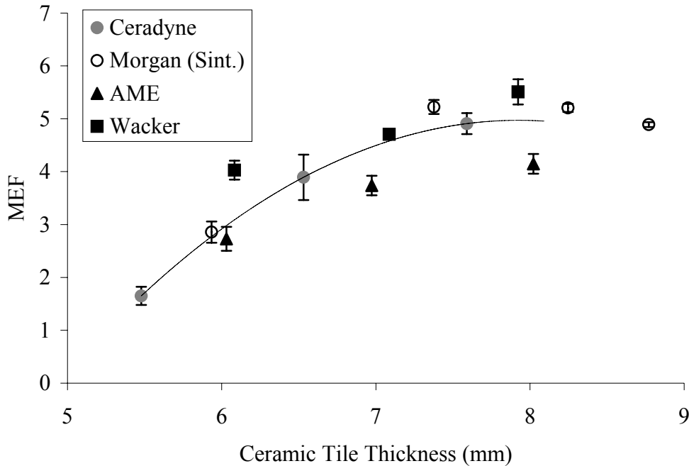
Figure 5: Effect of increasing thickness on the calculated mass efficiency factor for the ceramic.
