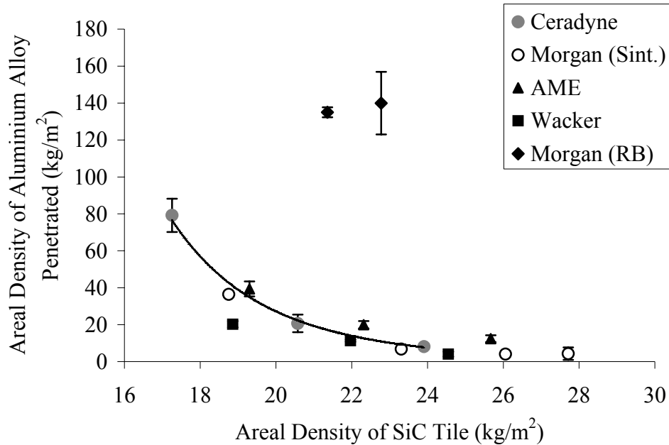
Figure 3: Reduction in areal density of Al6082 T651 penetrated with increasing silicon carbide tile areal density.
