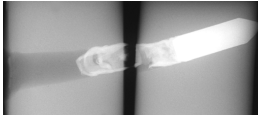
Figure 7: X-ray of the depth of penetration into the aluminium alloy witness block after completely penetrating 7.16mm of Morgan Reaction Bonded silicon carbide. Note that the core remains in tact.
