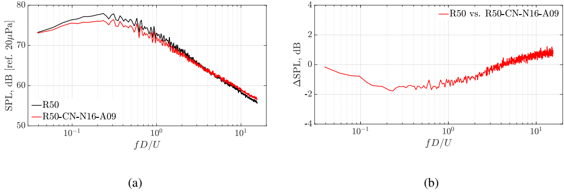
Figure 4: Far-field autospectra of the isolated baseline and chevron jets; [ \theta = 90^\circ , \varphi = 0^\circ , M_j = 0.6 ].
