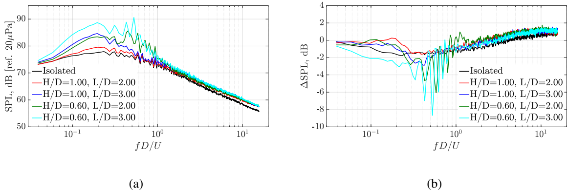
Figure 5: Far-field acoustic spectra [ \theta = 90^\circ , \varphi = 0^\circ , M_j = 0.6 ]. a) Sound pressure level of the installed R50 nozzle at varying jet-wing position; b) Delta sound pressure level between the chevron and baseline jets at varying jet-wing position.
