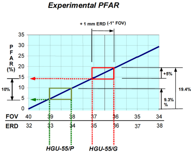
FIG. 15 Percentage variation of the PFAR as a function of ERD and FOV.
