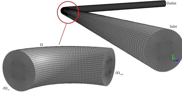
Figure 1: Schematic representation of the control volume \Omega of 90 0 bend
