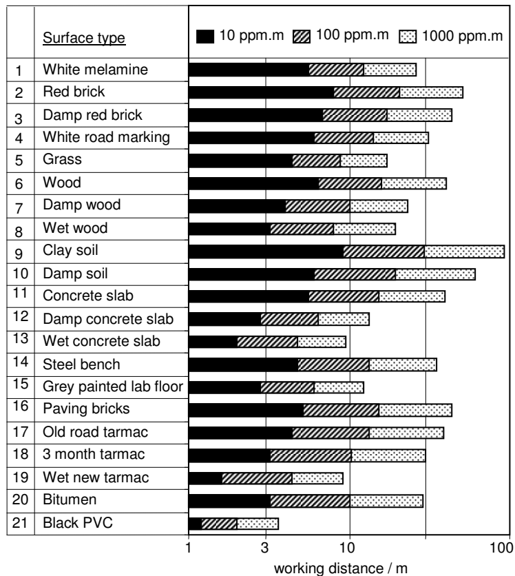
Figure 7. Range in metres at which a hypothetical laser pointer would detect a signal strength of 1000ppm.m, 100ppm.m and 10ppm.m, with a signal to noise ratio of unity, for different surface types.
