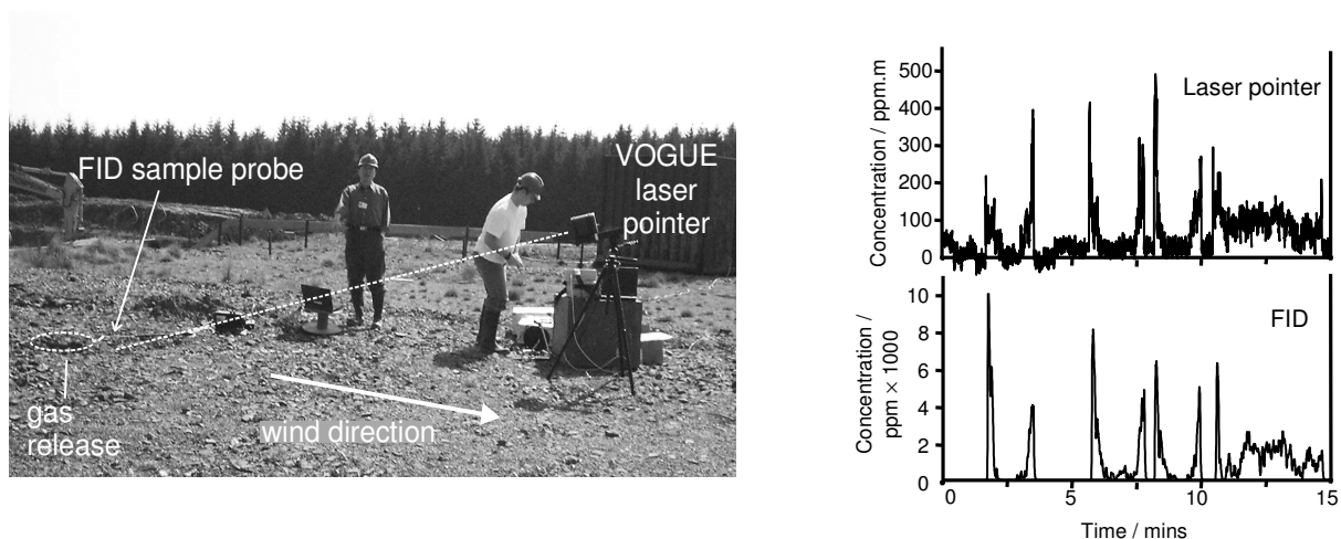
Figure 12. Correspondence between field measurements from a prototype laser pointer and flame ionisation detector targeted at the same sampling location, taken during a release of natural gas at 10 \text{ litre min}^{-1} .
