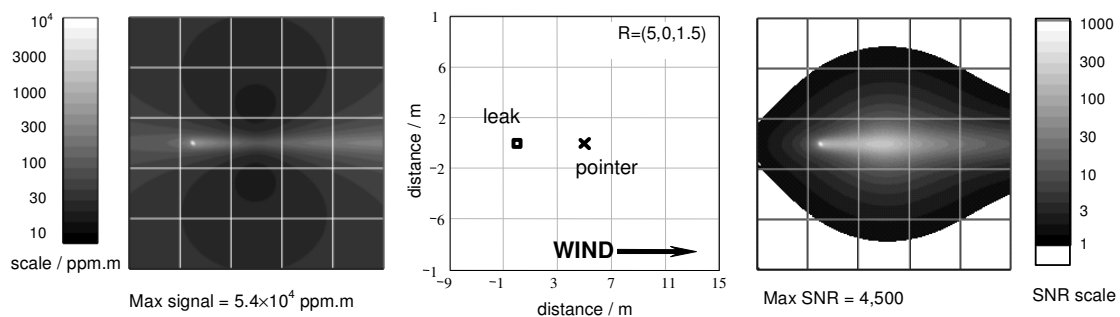
Figure 9(a). 5m away from the leak, a large maximum appears at the leak source with a lower, less well-defined maximum away from the source (surface: dry concrete).
