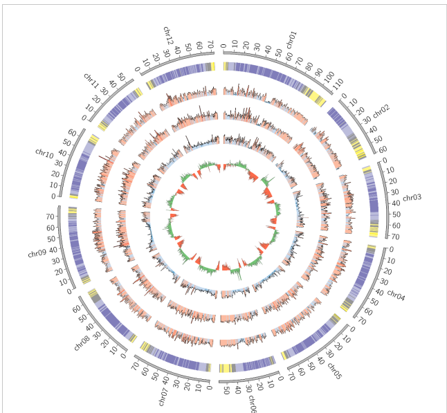
FIGURE 4 Circos plot of the final S. chilense assembly (scaffolds unmapped to pseudomolecules were omitted). From the outside to the inside, the layers are respectively representing chromosomes, gene density (purple = low density, yellow = high density), SNP density against S. lycopersicum , SNP density against S. pennellii , SNP density against S. chilense LA3111 (blue = low, red = high), and GC content (green = GC content above the genome mean GC content, red = GC content below the genome mean).
