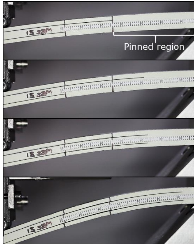
Figure 14 Delamination propagation sequence for pinned samples (Delaminations highlighted for clarity)
