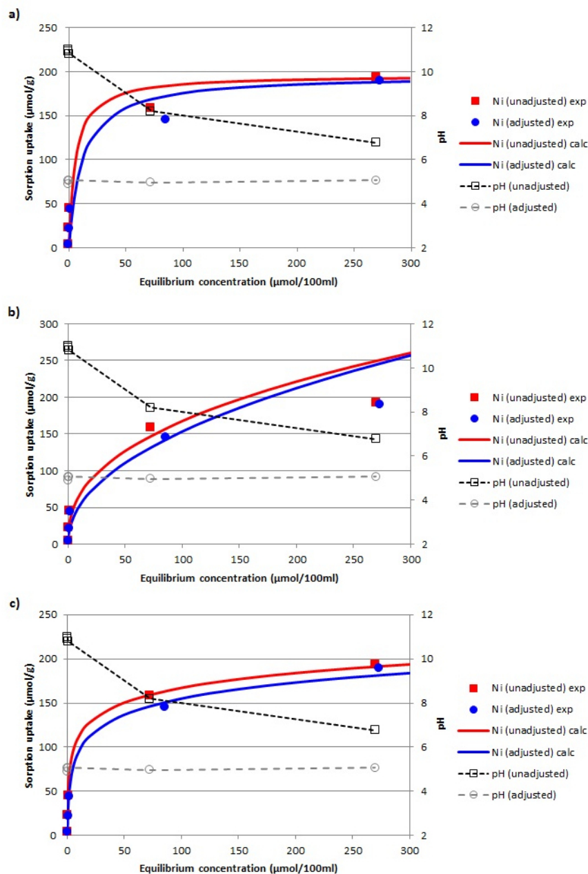
Figure 5: Experimental and simulated data proximity. Comparison between the experimental data (exp) and the simulated adsorption isotherms (calc) of \text{Ni}^{2+} onto the zeolitic material according to the (a) Langmuir, (b) Freundlich, and (c) Temkin models. Please click here to view a larger version of this figure.
