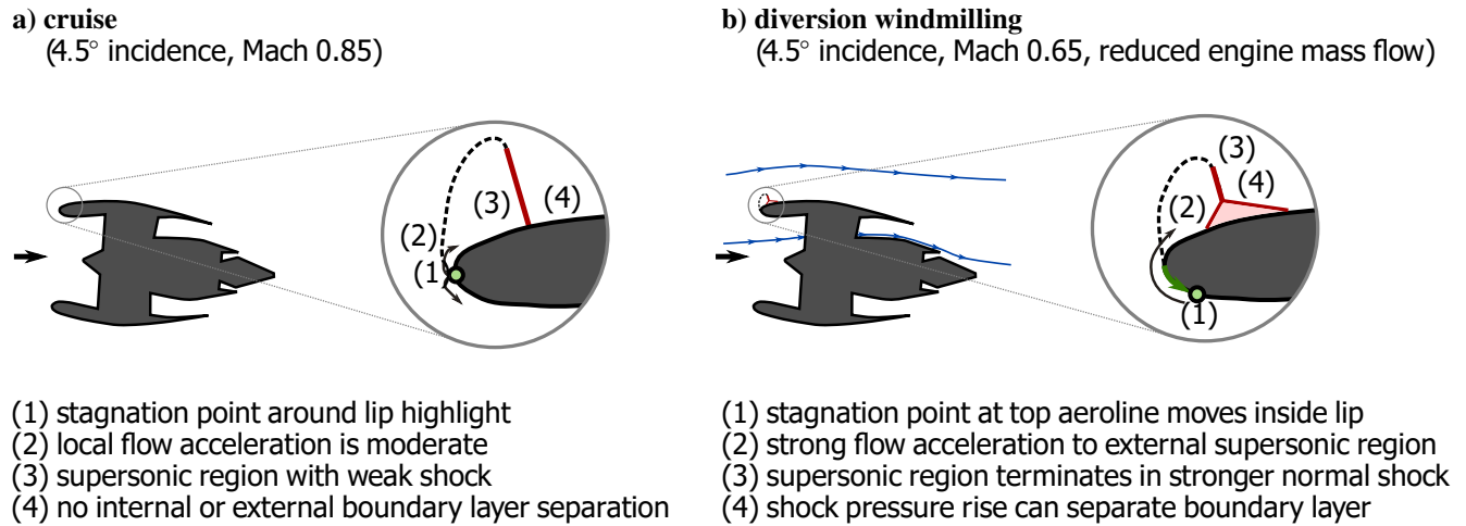
Fig. 1 Schematic of flow fields for (a) on-design cruise and (b) off-design diversion windmilling conditions.
