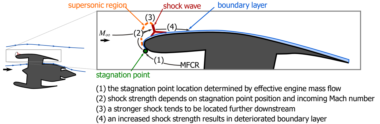
Fig. 22 Conceptual model summarising relationships between key flow parameters in the diversion windmilling flow field.
