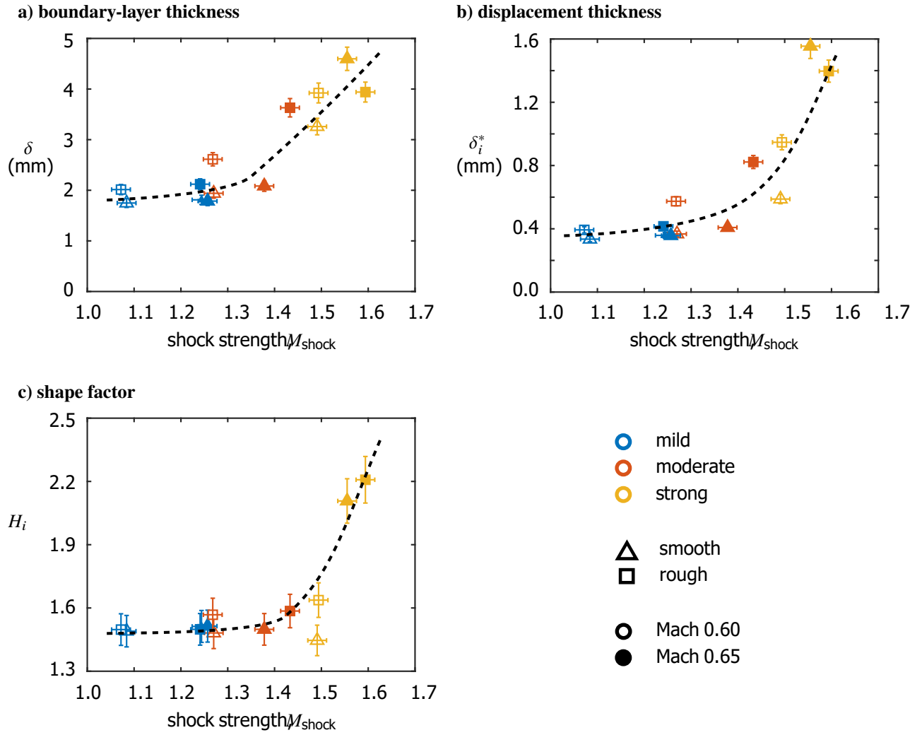
Fig. 19 Correlation between measured boundary-layer parameters and shock strength.
