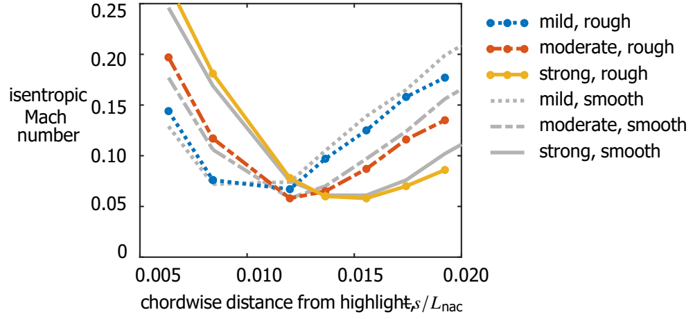
Fig. 15 Isentropic Mach number around the stagnation point for a rough surface at Mach 0.65, compared to the smooth case. Error bars are excluded for clarity but are consistent with those presented in Fig. 5.
