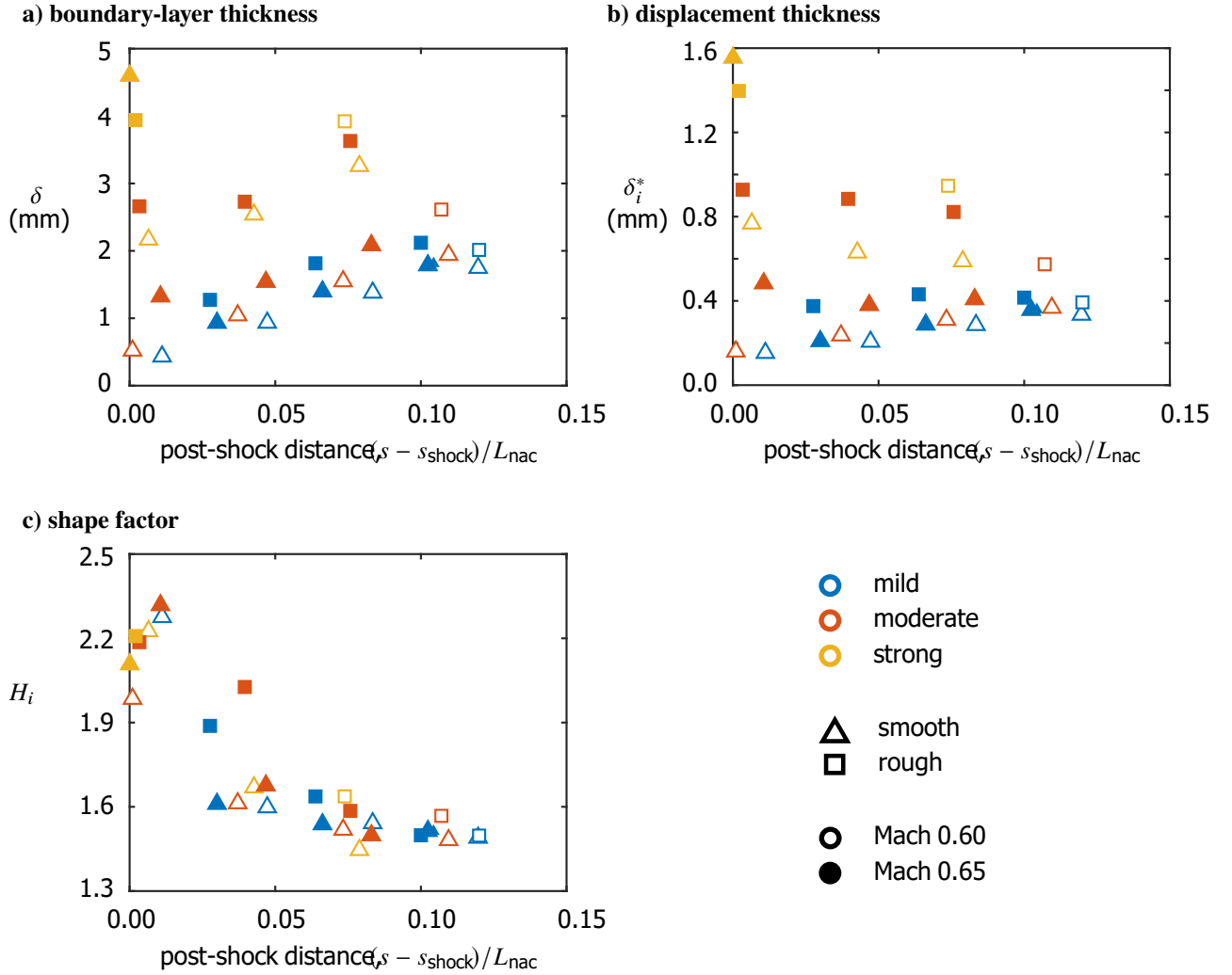
Fig. 23 Measured boundary-layer parameters as a function of post-shock distance.
