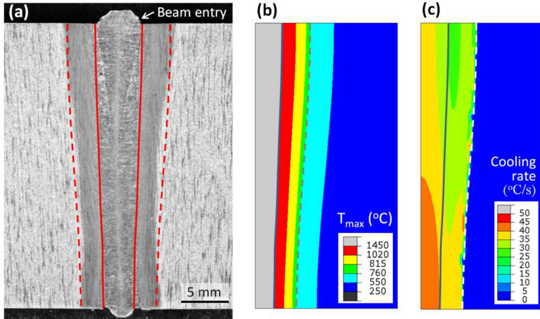
Fig. 5. (a) Mid-length macrograph of the EB weld; (b) predicted distribution of peak temperature; (c) predicted distribution of cooling rate at 700 °C. Note that the predicted isothermal lines that correspond to the FZ boundary (solid line) and HAZ boundary (dashed line) are superposed in the macrograph shown in (a).
