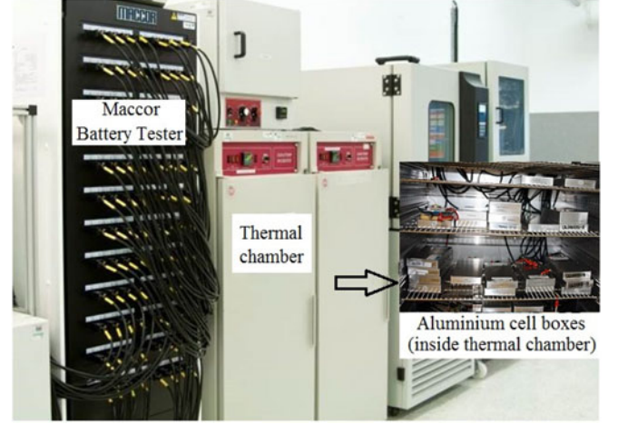
Fig. 5. Cell test equipment.
