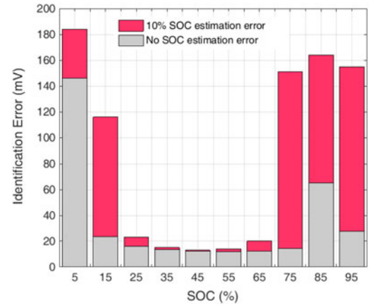
Fig. 16. Cell terminal voltage prediction error with and without SOC estimation error.
