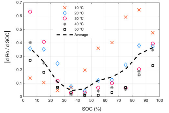
Fig. 15. Derivative of Li-S cell ohmic resistance over SOC at different charge and temperature levels.
