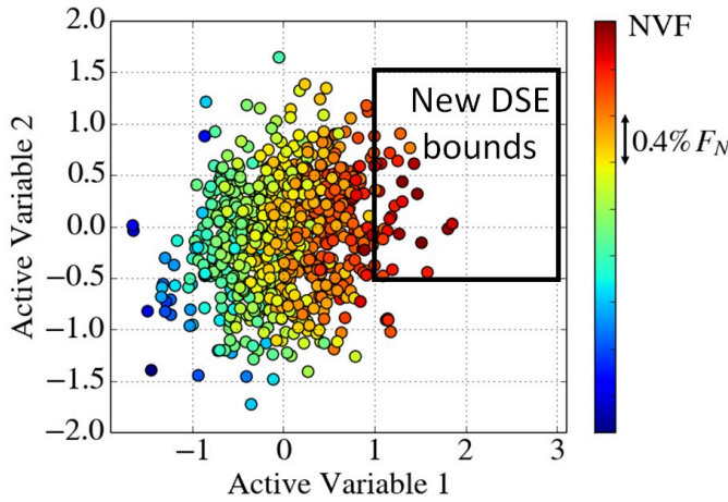
FIGURE 3: Projection of the 32 dimensional space into 2 after applying the active subspace method. The bounds of the new refined DSE are also marked
