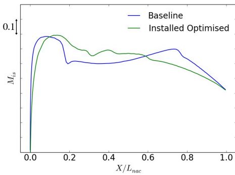
FIGURE 10: M_{is} comparison for selected nacelle aero-lines
