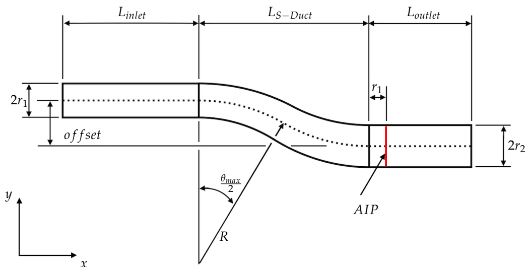
Figure 2. S-Duct scheme.
