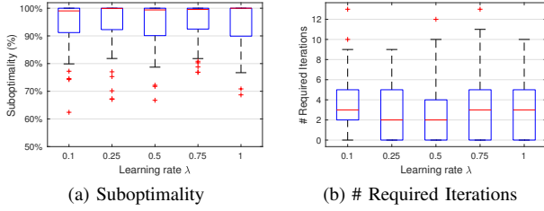
Fig. 1. Parametric analysis regarding the learning rate \lambda ( n_a = 10, n_t = 3 ) (a) the suboptimality (i.e., f_{opt}/f_A , where f_{opt} is the total cost by a brute-force algorithm and f_A is that by the proposed algorithm); (b) the number of iterations required for convergence to a Nash-stable partition.
