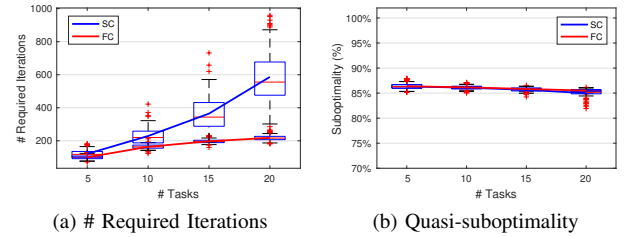
Fig. 4. Parametric analysis regarding n_t ( n_a = 100 )
