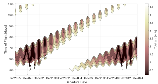
Figure 1: 1-revolution transfer opportunities to 2006 RH 120
