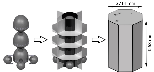
Figure 4: Fuel tanks and ZEUS-15 skeleton. Representation of how the tanks have driven the final dimensions of the S/C.
