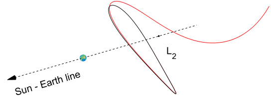
Figure 2: Insertion Halo Orbit at L_2 (black) and its associated manifold (red). The Earth's size is exaggerated for visualisation purposes.
