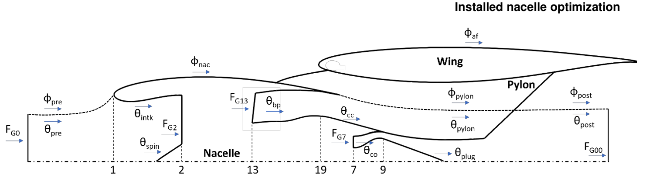
Figure 2 – Thrust and drag accounting method for the installed nacelle configuration.
