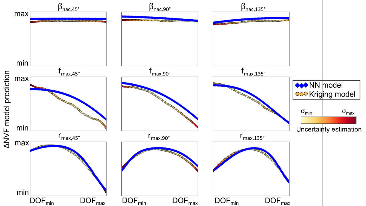
Figure 8 – 1-dimensional interrogation of the Kriging and ANN surrogate models in the analysed design space.
