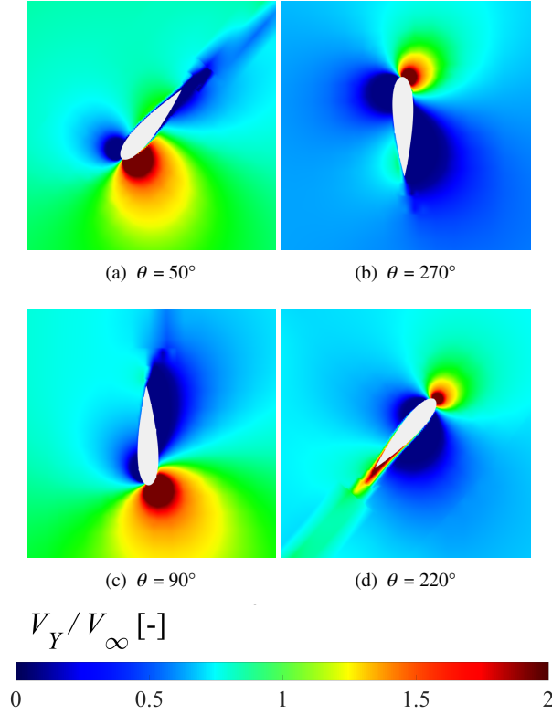
Fig. 8 Instantaneous streamwise velocities experienced by a VAWT blade at different azimuth locations for the VAWT configuration without struts and tower, using the high-fidelity LBM at \text{TSR} = 4
