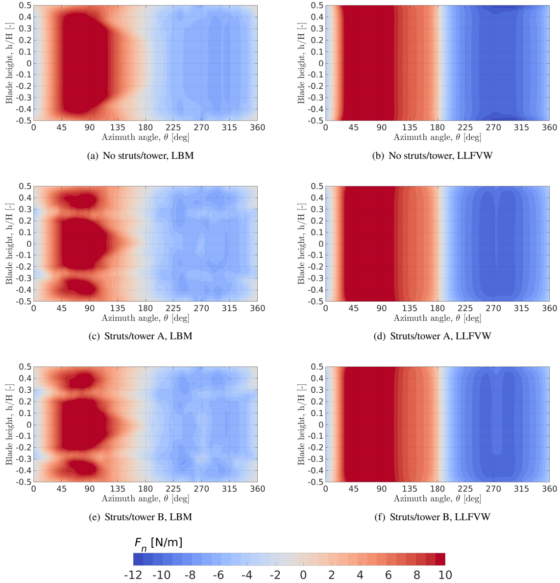
Fig. 12 Normal force contour for a single blade over azimuthal and spanwise directions, using the high-fidelity LBM and mid-fidelity LLFVW, at \text{TSR} = 4
