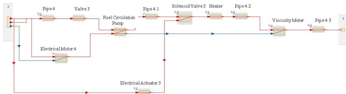
Fig. 7. Circulation unit functional model
