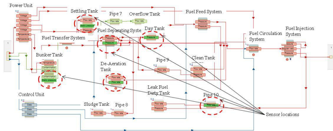
Fig. 10. PHM Sensor set solution
