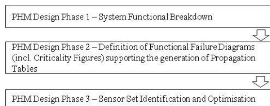
Fig. 3. PHM Design Process
