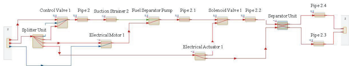
Fig. 5. MADe Separation unit functional model
