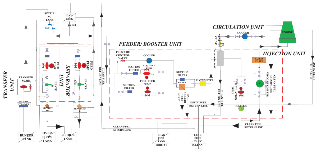
Fig. 2. Fuel system – Sub-system and component level breakdown (adapted from [17])
