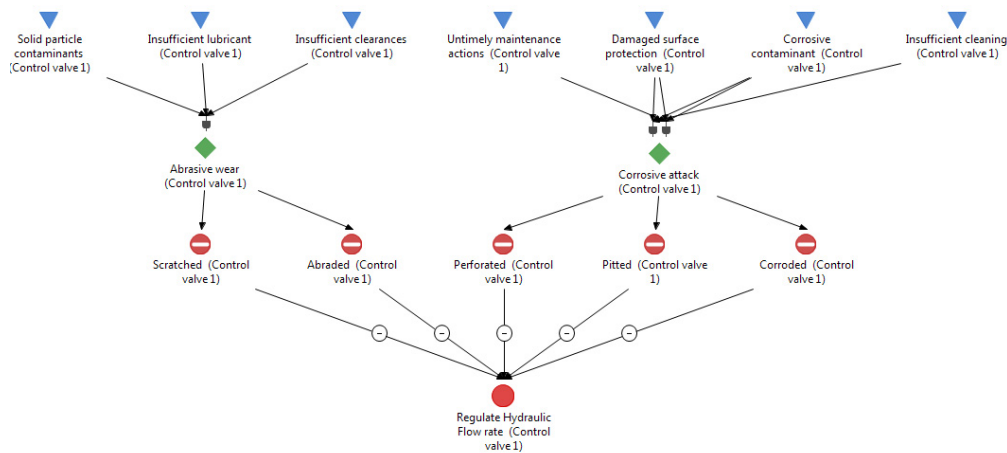
Fig. 9 Control valve - Failure diagram (incl. causes, mechanism, faults and the functional failures)
