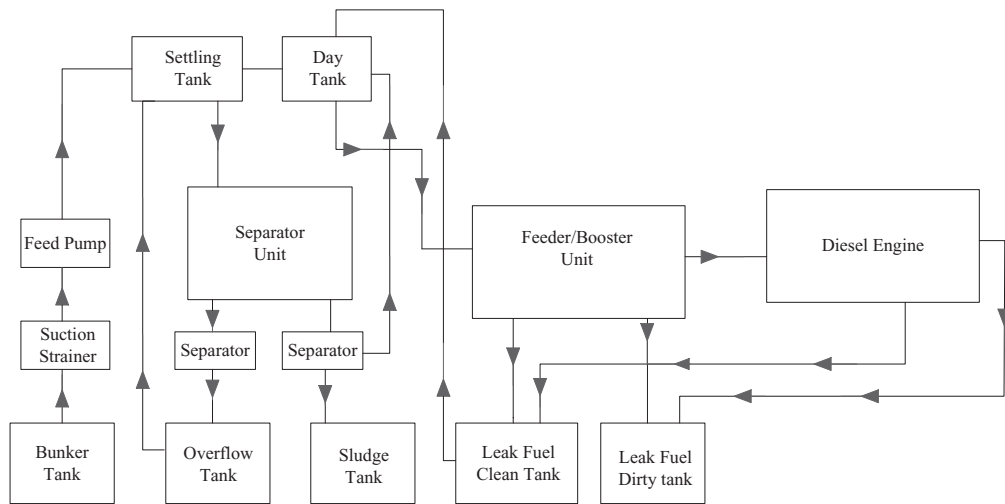
Fig. 1. Fuel system – High Level Block Diagram (adapted from [8])
