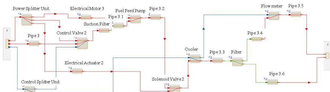
Fig. 6. Feed unit functional model
