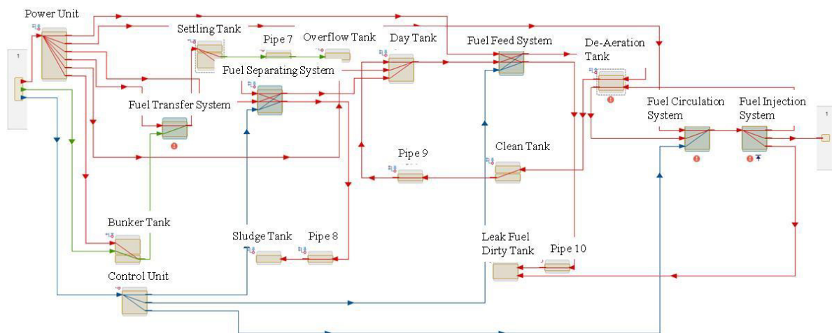
Fig. 4. MADe Fuel system functional model
