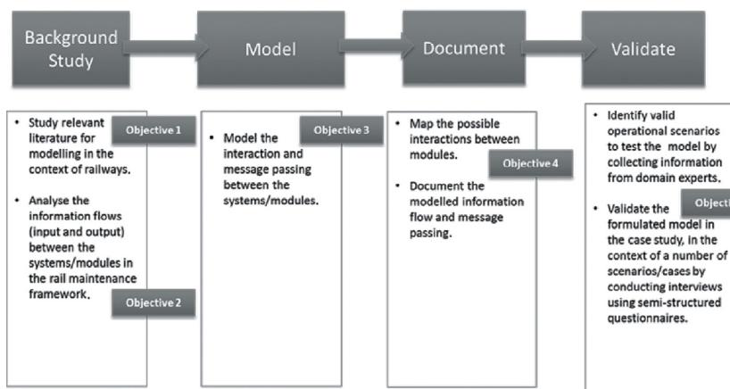
Figure 1: Methodology employed.
