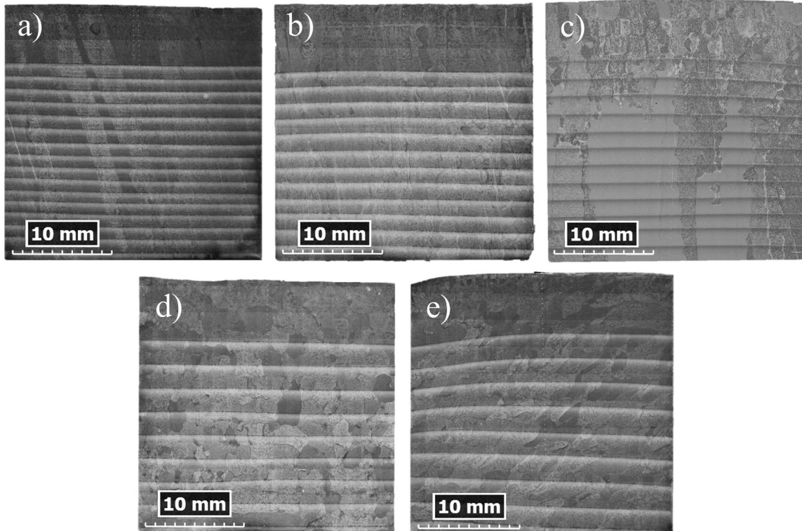
Fig. 2. Etched macrographs of Ti-6Al-4V specimens 1–5 illustrating change in prior- \beta grain morphology changes as SED of deposited material is reduced a) 37.93 J.mm -3 , b) 30.39 J.mm -3 , c) 28.48 J.mm -3 , d) 22.28 J.mm -3 , e) 21.64 J.mm -3 .
