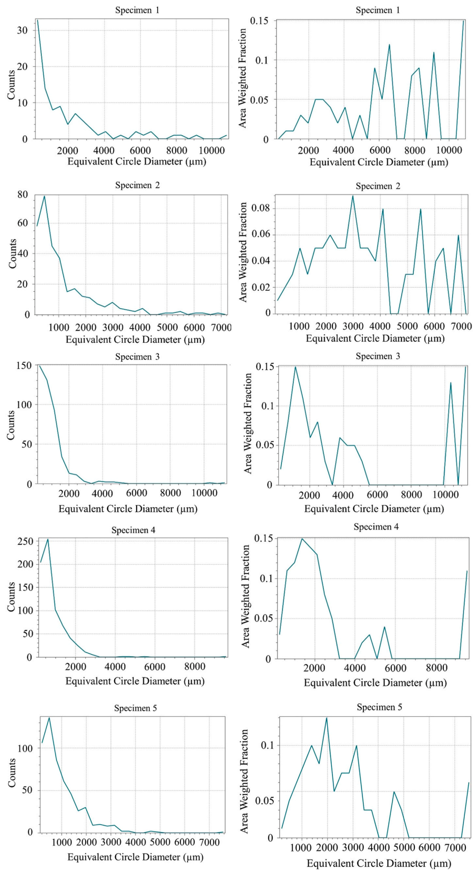
Fig. 9. Grain size distribution of specimens 1–5. (L) Number of counted grains (R) Area weighted distribution of grain size.
