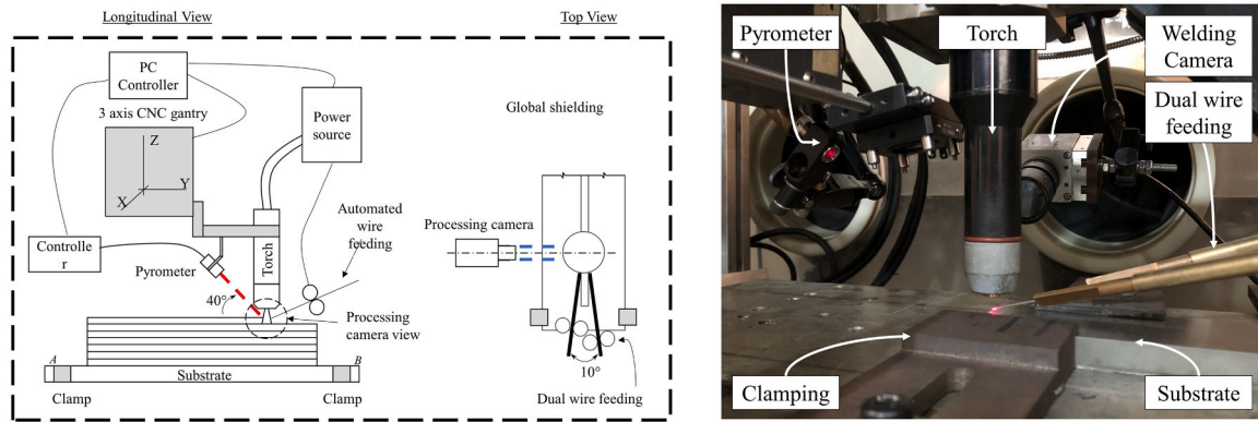
Fig. 1. (L) Schematic of experimental setup. (R) Experimental Setup.
