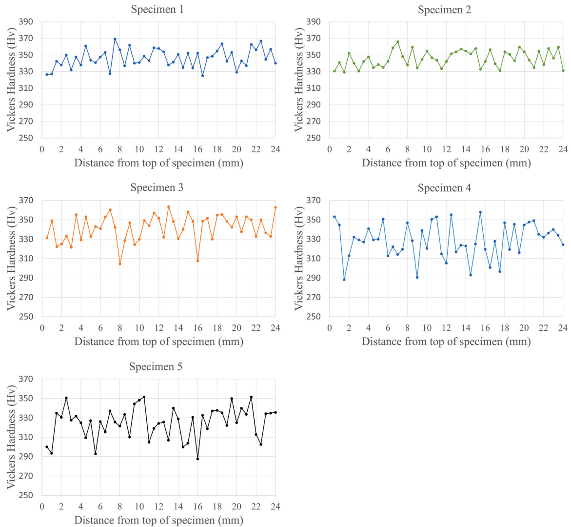
Fig. 11. Microhardness (HV0.3) measurements of specimens 1–5 - (1) 37.93 J.mm -3 (2) 30.39 J.mm -3 (3) 28.48 J.mm -3 (4) 22.28 J.mm -3 (5) 21.64 J.mm -3 .
