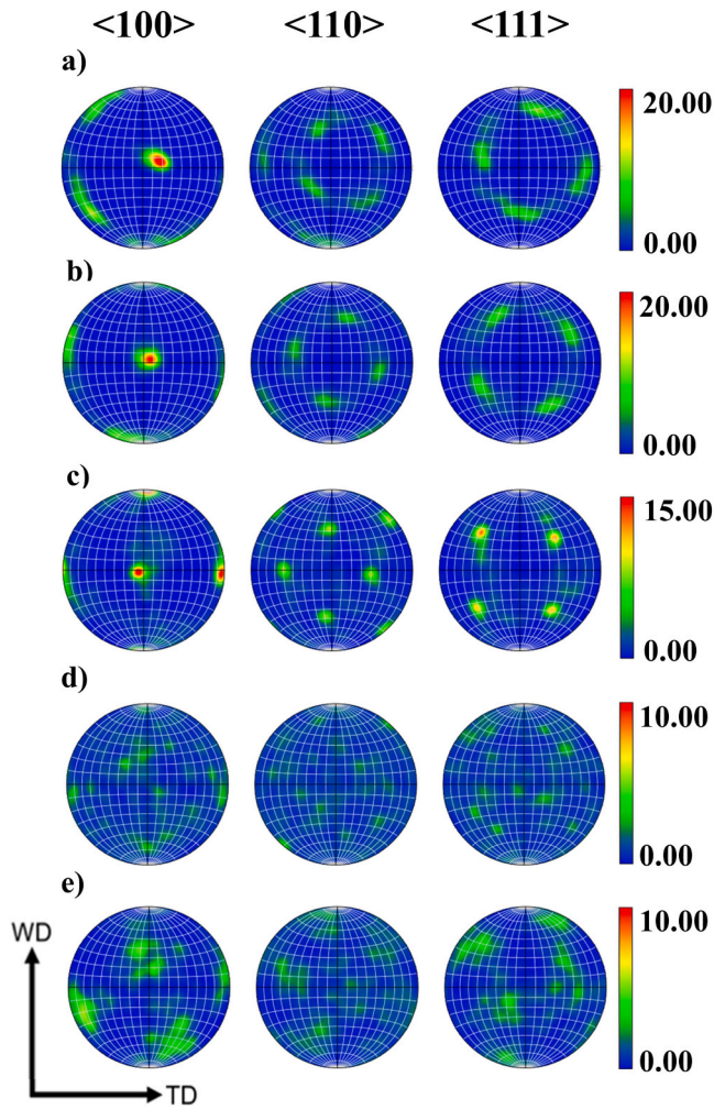
Fig. 8. Pole figures of specimens 1–5 indicating crystallographic texture a) 37.93 J.mm -3 b) 30.39 J.mm -3 , c) 28.48 J.mm -3 , d) 22.28 J.mm -3 , e) 21.64 J.mm -3 .
