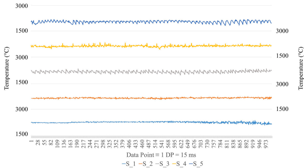
Fig. 6. Real-time pyrometric recording for specimens 1–5 (ascending). (15 ms interval time per data point.) Specimen layers: 31, 23, 23, 17, 16 respective to Fig. 5 observed transfer modes.
