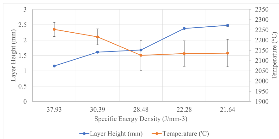
Fig. 4. Effect of SED on layer height and recorded temperature during deposition.
