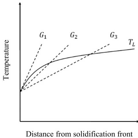
Fig. 3. Illustration outlining the effect of how a reduction in thermal gradient increases the total amount of undercooling by increasing the total area created by the liquidus temperature line ( T_L ) and dashed thermal gradient line. *Note that here the curvature of T_L does not represent Ti-6Al-4V and is inflated for the purpose of explanation.
