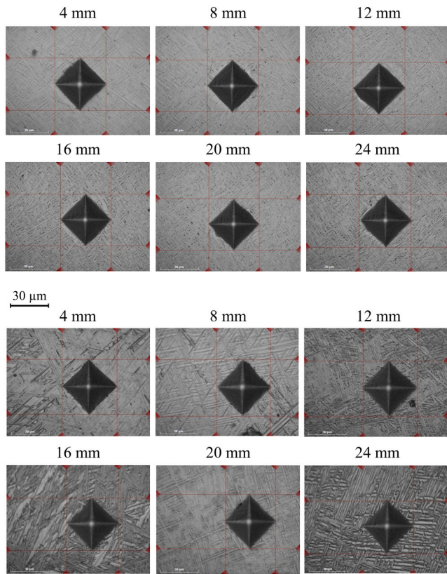
Fig. 12. Vickers hardness indentations showing localised microstructure of specimen 1 (columnar prior- \beta grains) and specimen 5 (refined prior- \beta grains) at 4 mm spacing below the top of the deposit.
