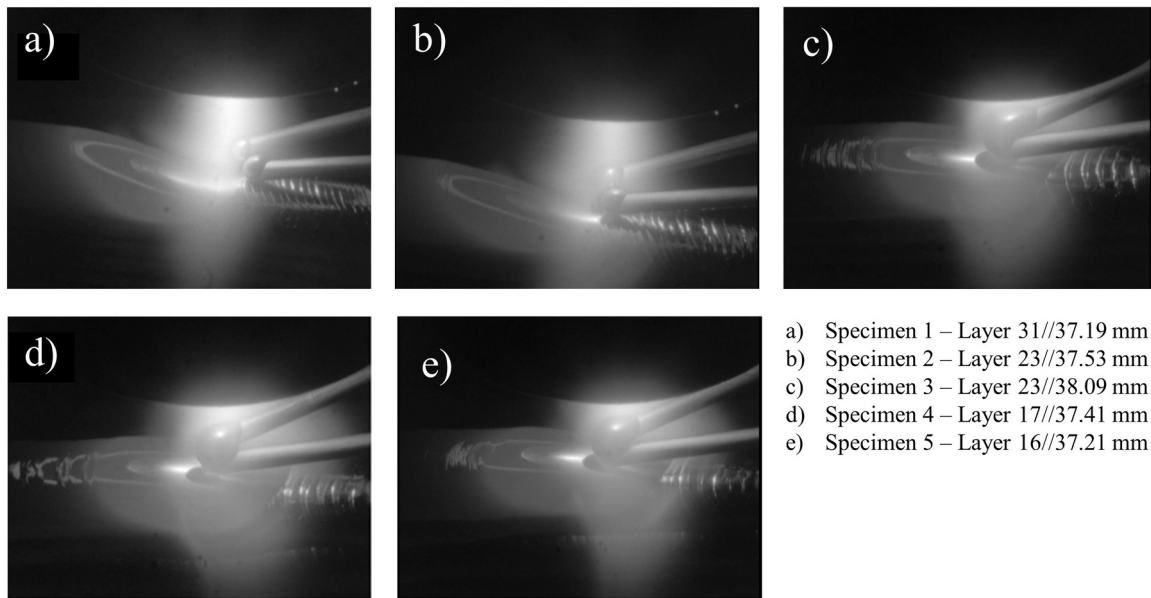
Fig. 5. Droplet transfer mode during deposition. a) 37.39 \text{ J.mm}^{-3} – TM2, b) 30.39 \text{ J.mm}^{-3} – TM2, c) 28.48 \text{ J.mm}^{-3} – TM3, d) 22.28 \text{ J.mm}^{-3} – TM3, e) 21.64 \text{ J.mm}^{-3} – TM3 at \sim 38 \text{ mm} build height.
