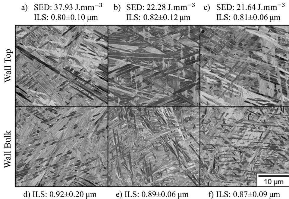
Fig. 10. Back-scattered electron images of \alpha lamellar microstructure and measured ILS for Specimens 1,4 and 5 respectively a)-c) wall top, d)-f) wall bulk.
