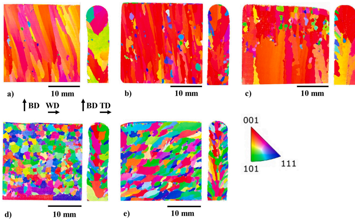
Fig. 7. EBSD IPF maps of specimens 1–5 with reducing SED, a) 37.93 J.mm -3 , b) 30.39 J.mm -3 , c) 28.48 J.mm -3 , d) 22.28 J.mm -3 e) 21.64 J.mm -3 , showing the transition from a columnar grain structure to a refined one in both the longitudinal and transverse plane.
