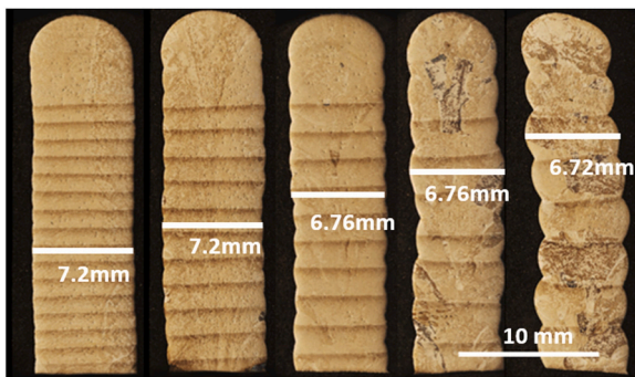
Fig. 13. Change in wall width and surface roughness as SED is reduced from 37.93 J.mm -3 (left), 30.39 J.mm -3 , 28.48 J.mm -3 , 22.28 J.mm -3 , 21.64 J.mm -3 (right).
