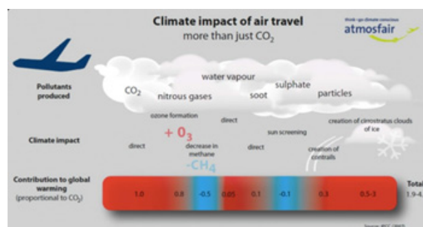
Figure 1 Climate impact on air travel.
