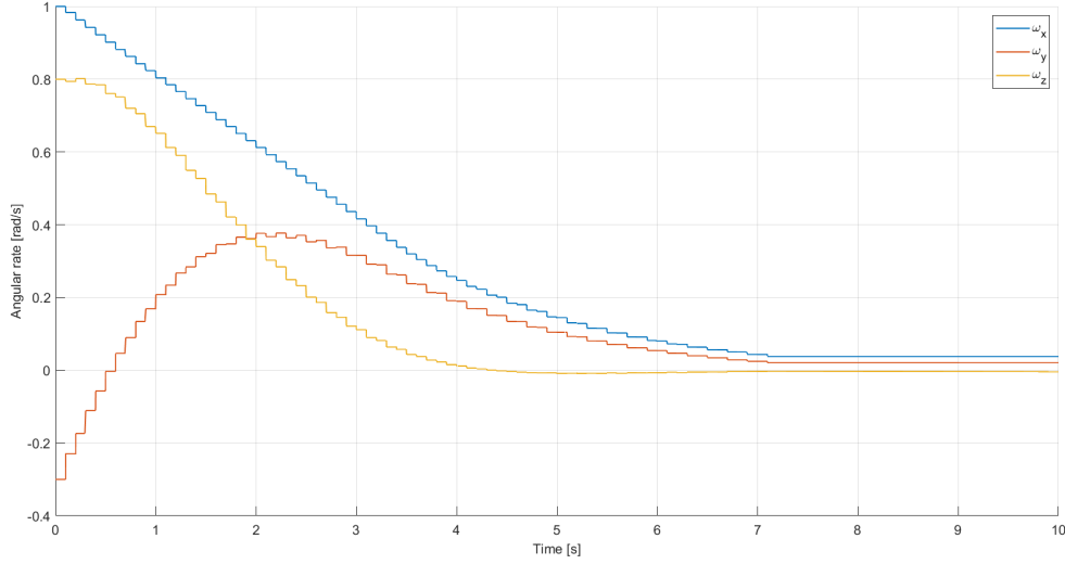
Fig. 3 Dynamics stability
