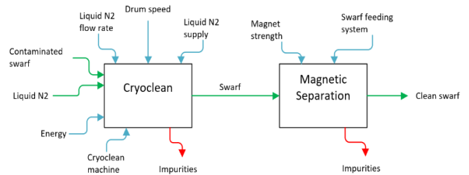
Fig. 2. Cryoclean process map.
