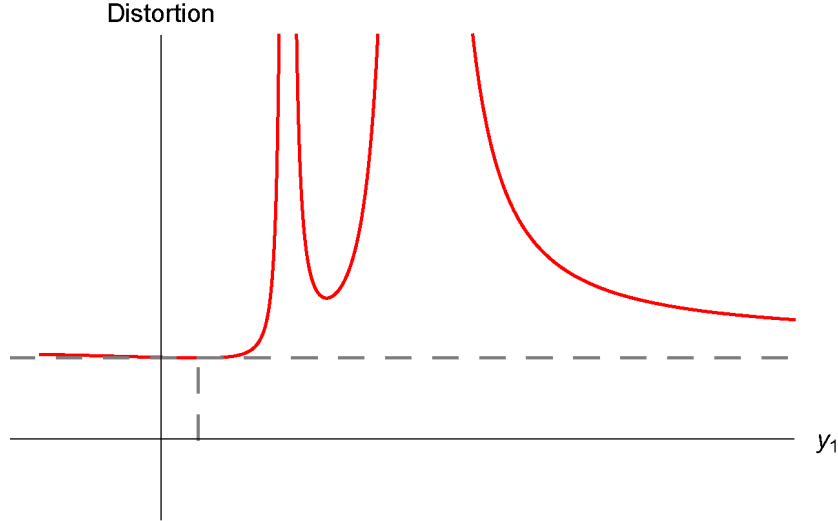
Figure 3: Possible trend of the distortion in Eq. (34) as a function of y_1 . Global minimum is identified by dashed lines.
