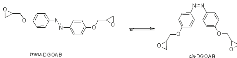
Fig. 1. Trans and cis isomeric forms of 4, 4'-diglycidyloxyazobenzene (DGOAB).
