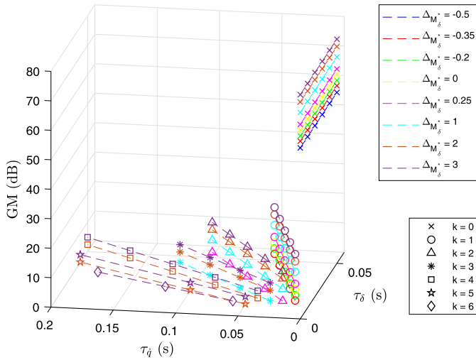
Fig. 3. Gain margin (GM) for stable closed-loop system under \tau_q and \tau_\delta together with \Delta\hat{M}_\delta^* .
