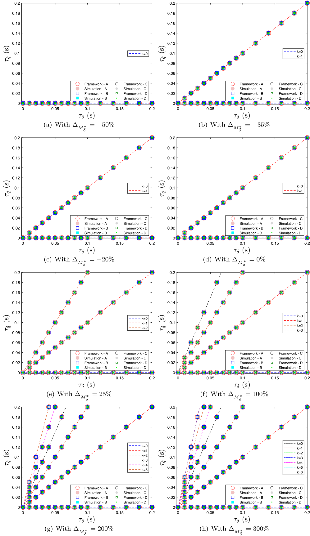
Fig. 1. Relationships between \tau_{\dot{q}} and \tau_{\delta} for system stability under \Delta_{M_{\delta}^*} . (For interpretation of the colours in the figure(s), the reader is referred to the web version of this article.)
