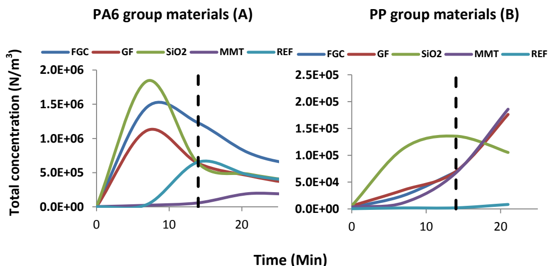
Figure 1. Monitoring of airborne NP using SMPS during 28 minutes of drilling. The concentration of NP generated from PA6 group materials shown in A; the concentration of NP generated from PP group materials shown in B. The lines represent NP released from polymer composites with reinforcement material of foam glass crystal (FGC), glass fiber (GF), silica NP (SiO2), montmorillonite (MMT), or without reinforcement material (REF).
