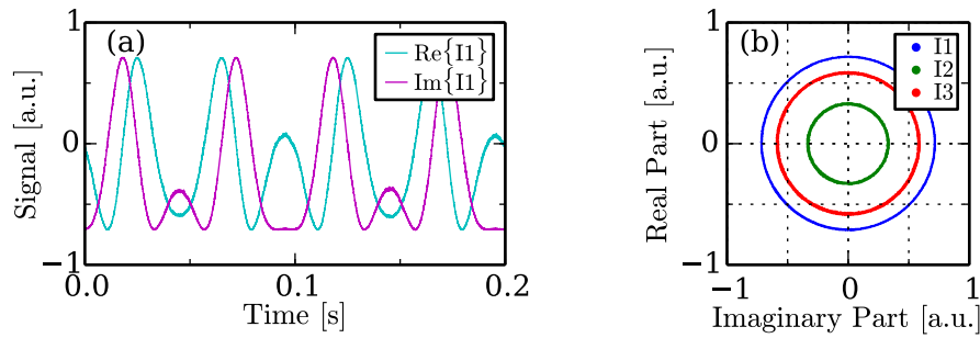
Fig. 8. The low-pass filtered, complex quadrature signal Q(t) is shown in (a) as a time series over 0.2 s for I1 without any corrections discussed previously in Sec. 3.2, while (b) shows the polar plots of all three constituent interferometers in the complex plane.
