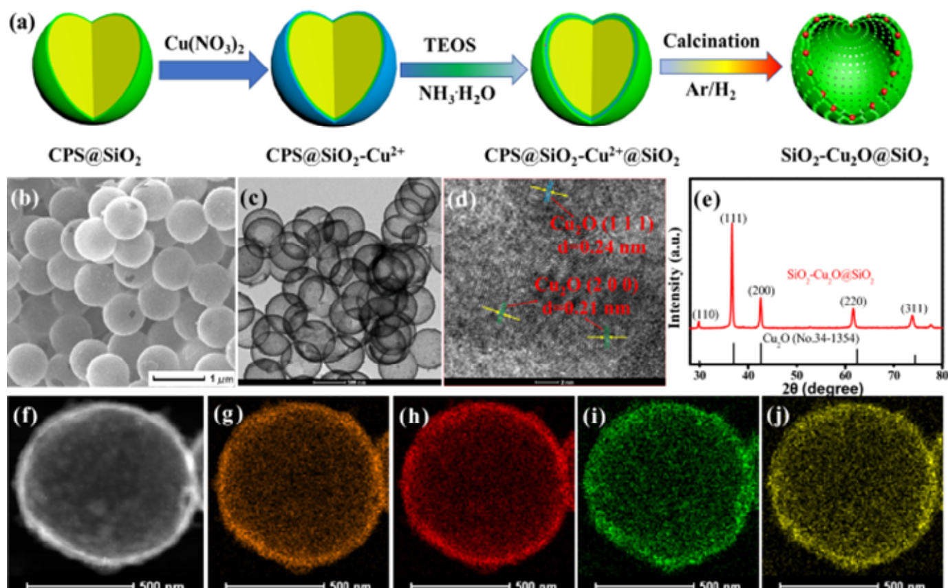
Figure 1. a The preparation process of the \text{SiO}_2\text{-Cu}_2\text{O@SiO}_2 photocatalyst.
