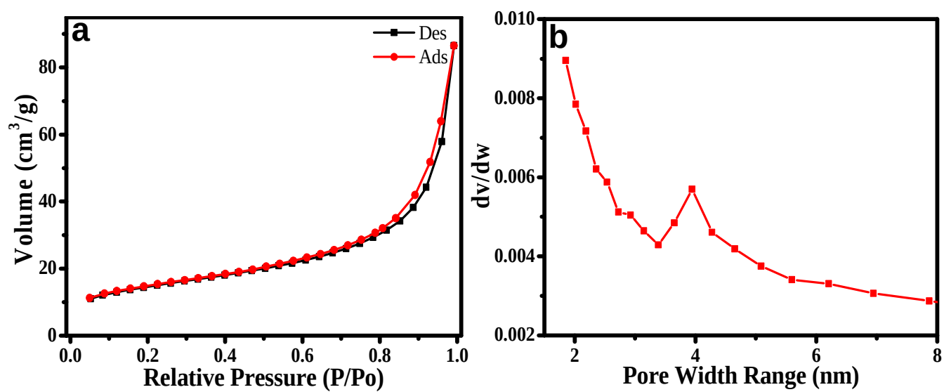
Fig.S3 N_2 adsorption-desorption isotherm (a) and pore size distribution (b) of the as-synthesized SiO_2-Cu_2O@SiO_2 photocatalyst
