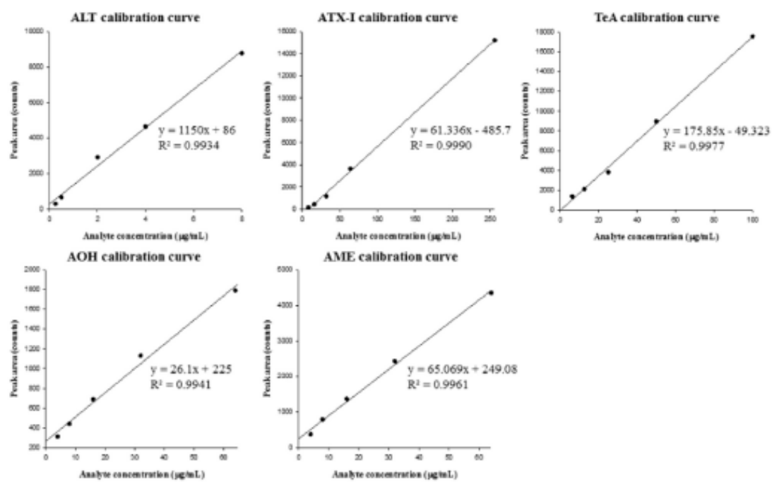
Fig. 6. Standard calibration curves for Alternaria mycotoxins: ALT, ATX-I, TeA, AOH, AME.
