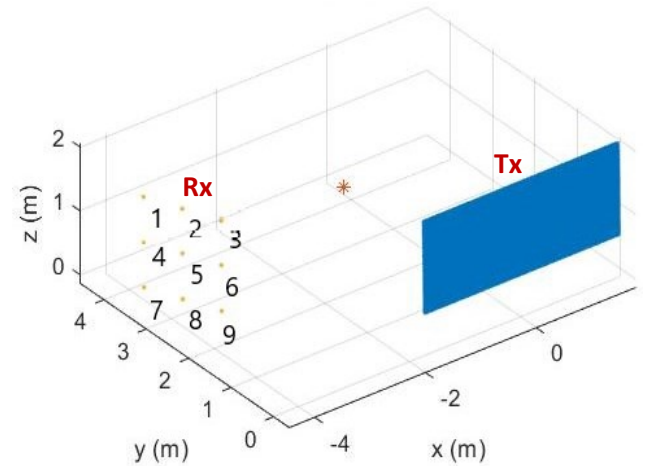
Fig. 2 Multistatic 3D SAR geometry, with 2D SAR aperture transmitter trajectory in blue, and nine fixed receiver positions to the left of the scene.
