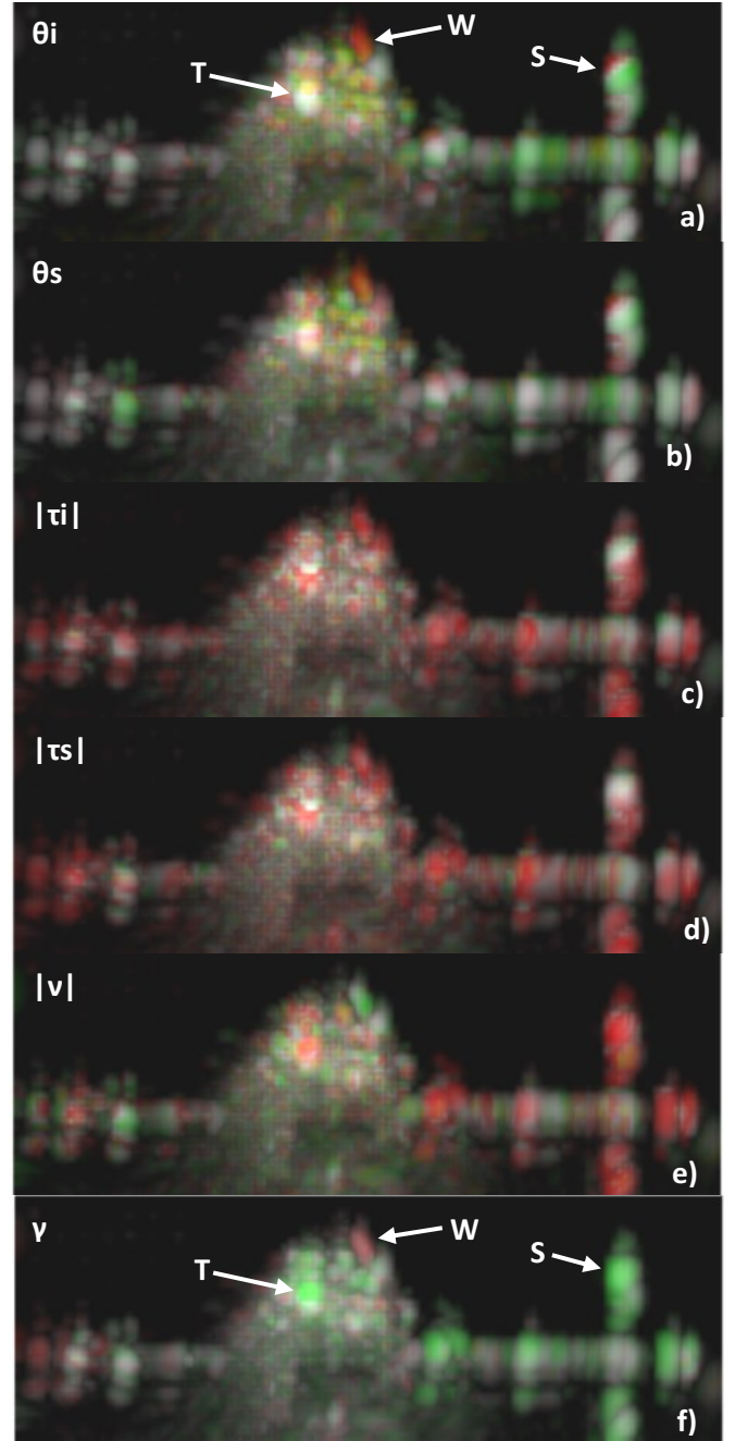
Fig. 7. Front-view polarimetric decomposed MIPs showing \theta_i , \theta_s , |\tau_i| , |\tau_s| , |v| , \gamma in a) to f) respectively, with colour maps presented in Fig. 8.
