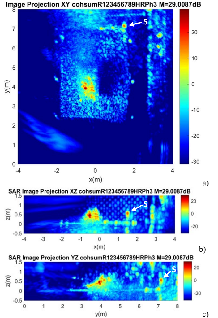
Fig 5. MIPs of a phase corrected coherent sum of the nine VV polarization 3D bistatic SAR images, with a z-projections (a), y-projection (b) and an x-projection (c). The large reference sphere is marked “S”.
