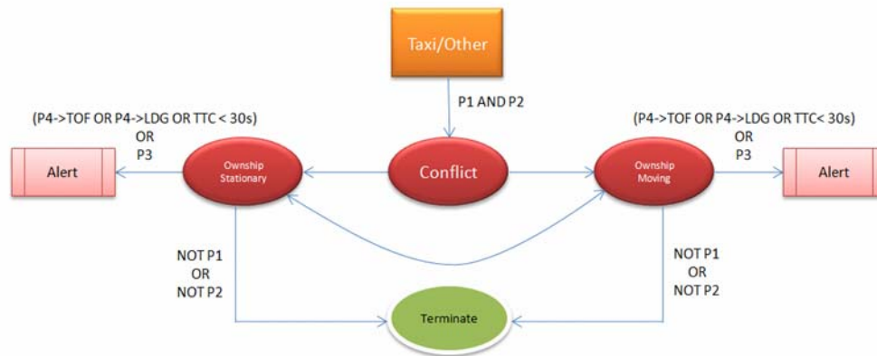
Figure 6 - State diagram for backtracking/line-up incursion alerting.
