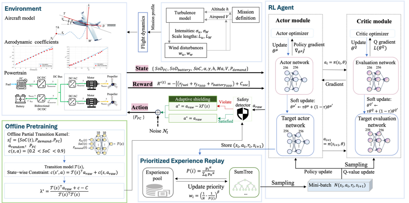
Fig. 7. Schematic of the LC-SEMS framework.
