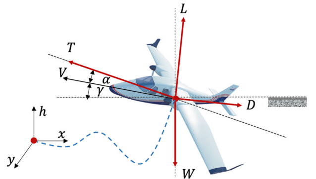
Fig. 1. Aircraft forces and position coordinate frame.
