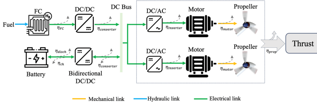
Fig. 3. Hybrid propulsion architecture.
