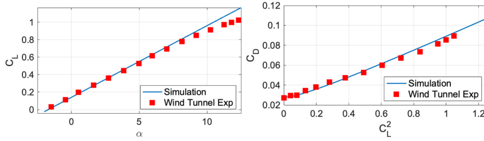
Fig. 2. Aerodynamic validation.
