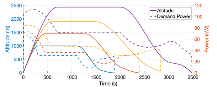
Fig. 8. Flight mission profile.
