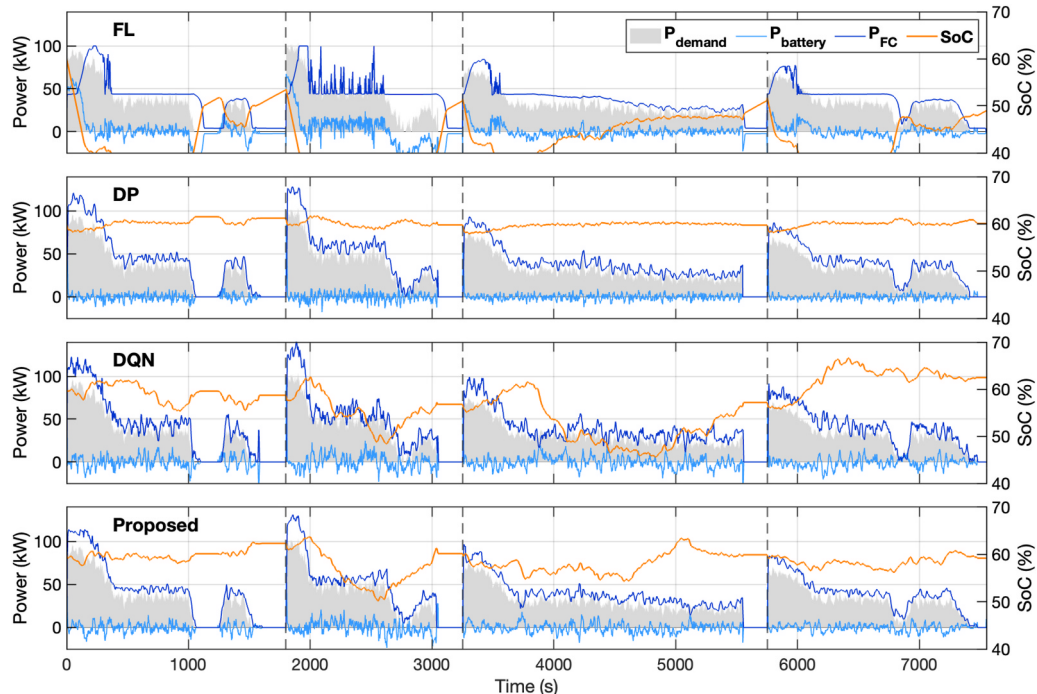
Fig. 12. Power distribution and SoC trajectory.
