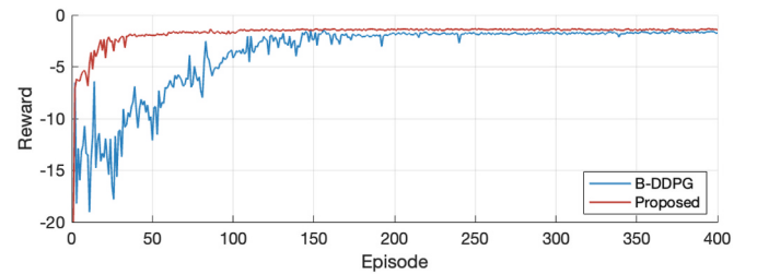
Fig. 10. Discounted reward of RL-based EMS.
