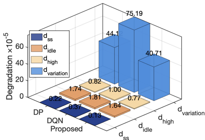
Fig. 15. FC degradation breakdown.
