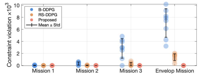
Fig. 11. Cumulative constraint violations of RL-based EMS.
