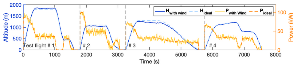
Fig. 9. Sequential Validation mission profile.
