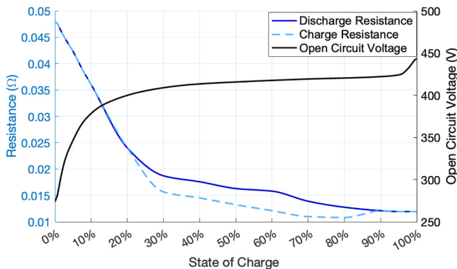
Fig. 4. Internal resistance and open circuit voltage of the battery.
