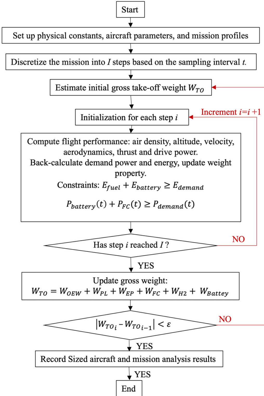
Fig. 5. Flow chart of hybrid electric aircraft mission analysis.
