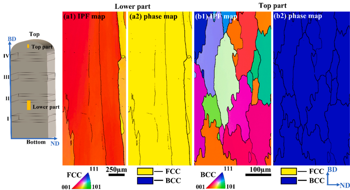
Fig. 5. EBSD orientation maps and phase maps of the PB-WDED \text{Al}_x\text{CoCrFeNi} HEA FGM component taken at the lower and top parts are displayed in (a1-a2) and (b1-b2), respectively. The crystal orientation-colour relation map corresponds to the inverse pole figure (IPF) legend. The FCC phase was highlighted in yellow, while the BCC phase was marked in blue. Note that the relationship between sampling and coordinates (building (BD), normal (ND), and transverse (TD) directions) are indicated on the right bottom.
