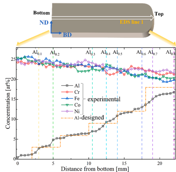
Fig. 2. Composition transition checked at the central line along BD of \text{Al}_x\text{CoCrFeNi} HEA functionally graded component deposited by PB-WDED method.
