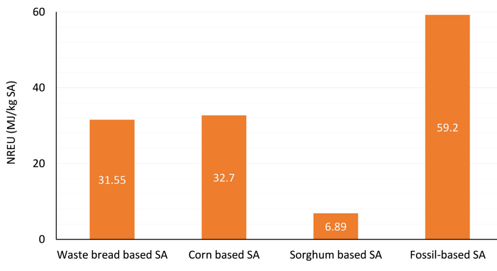
Fig. 5. Comparison analysis of NREU (MJ) of 1 kg SA production from three biomass-based substrates, bread waste, dextrose and sorghum grains, and the traditional petrochemical route.
