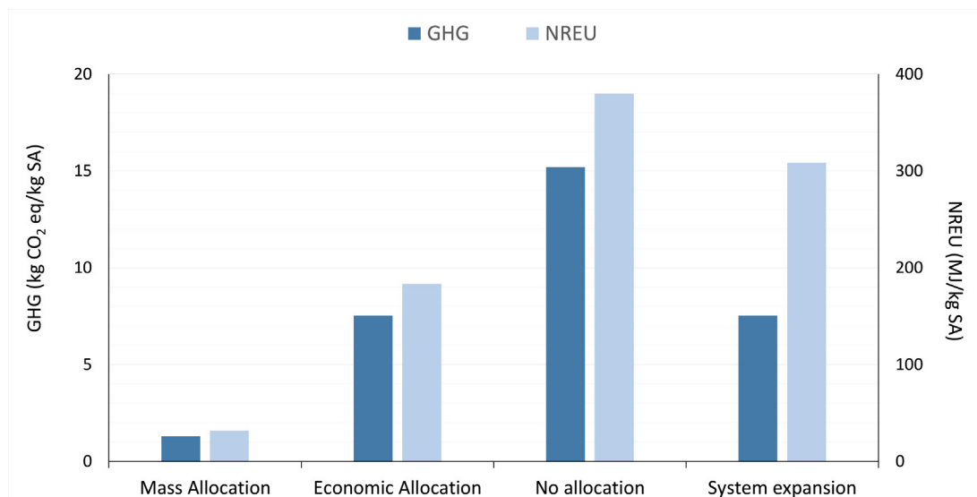
Fig. 6. Life cycle impact assessment results in terms of GHG emissions and NREU of SA production by fermentation of bread waste using different approaches to account for by-product.
