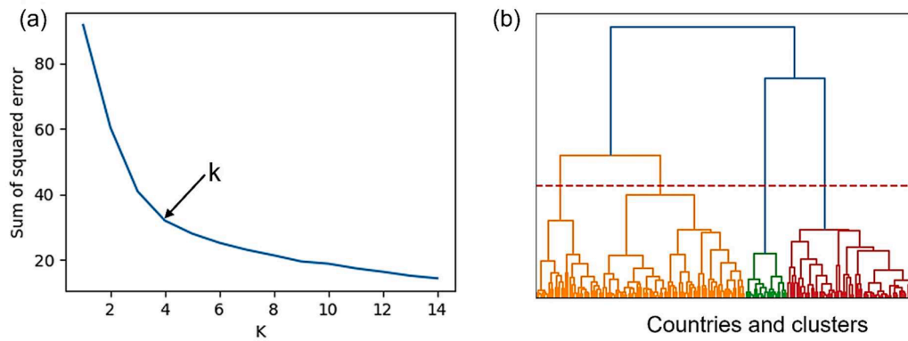
Fig. 2. (a) Optimum number of clusters ( k ) determined by the elbow method, (b) Forestation dendrogram.
