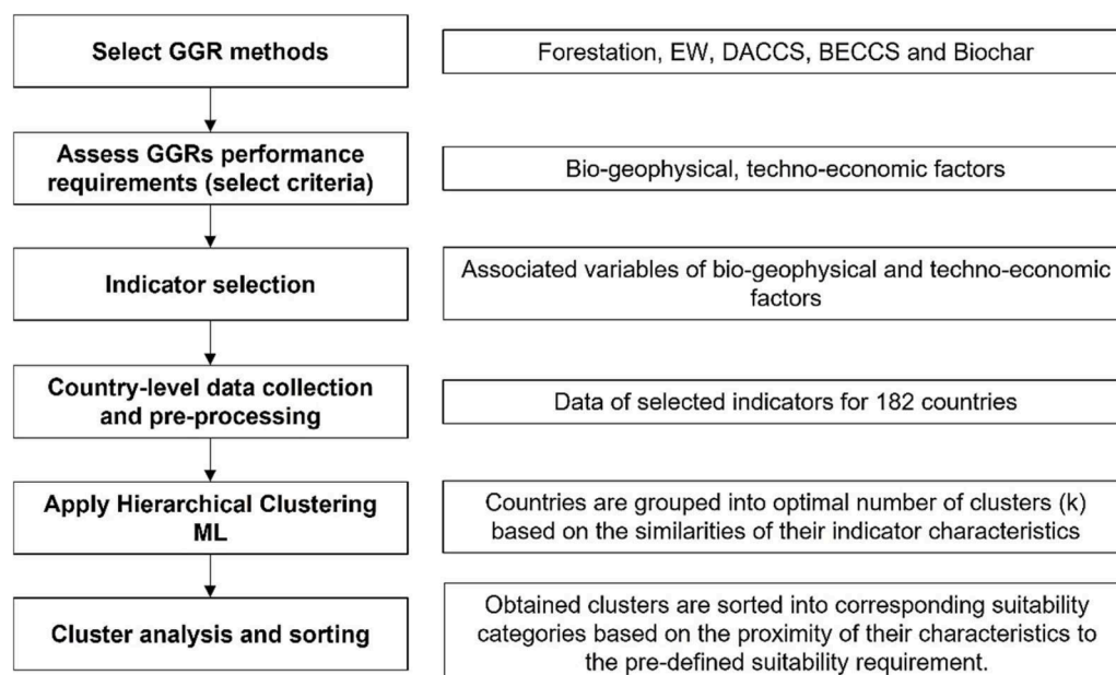
Fig. 1. Methodology framework for the study.
