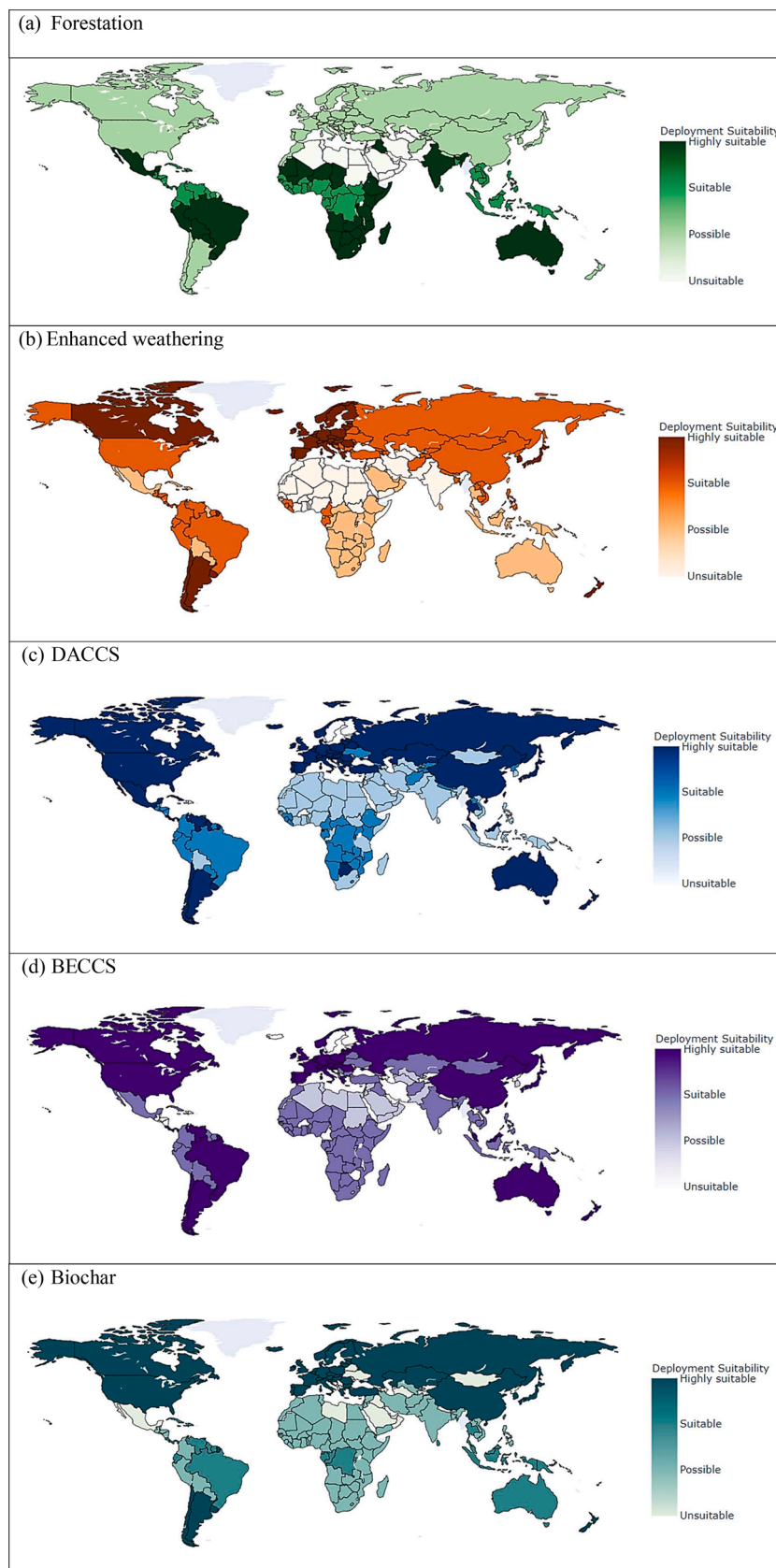
Fig. 4. Global maps showing the suitability of countries to deploy five GGR methods: Forestation (a), Enhanced weathering (b), DACCS (c), BECCS (d) and Biochar (e).
