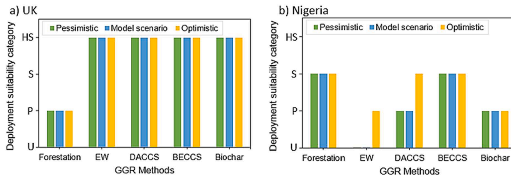
Fig. 6. Impact of model input variation (pessimistic and optimistic scenarios) on the deployment suitability categorisation of the UK and Nigeria.
