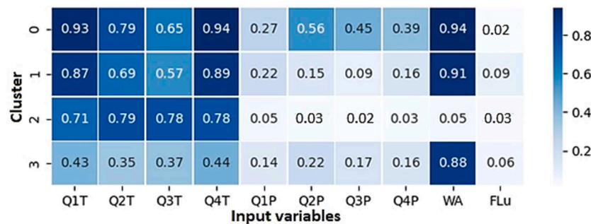
Fig. 3. Heat map showing the cluster characteristics for forestation.
