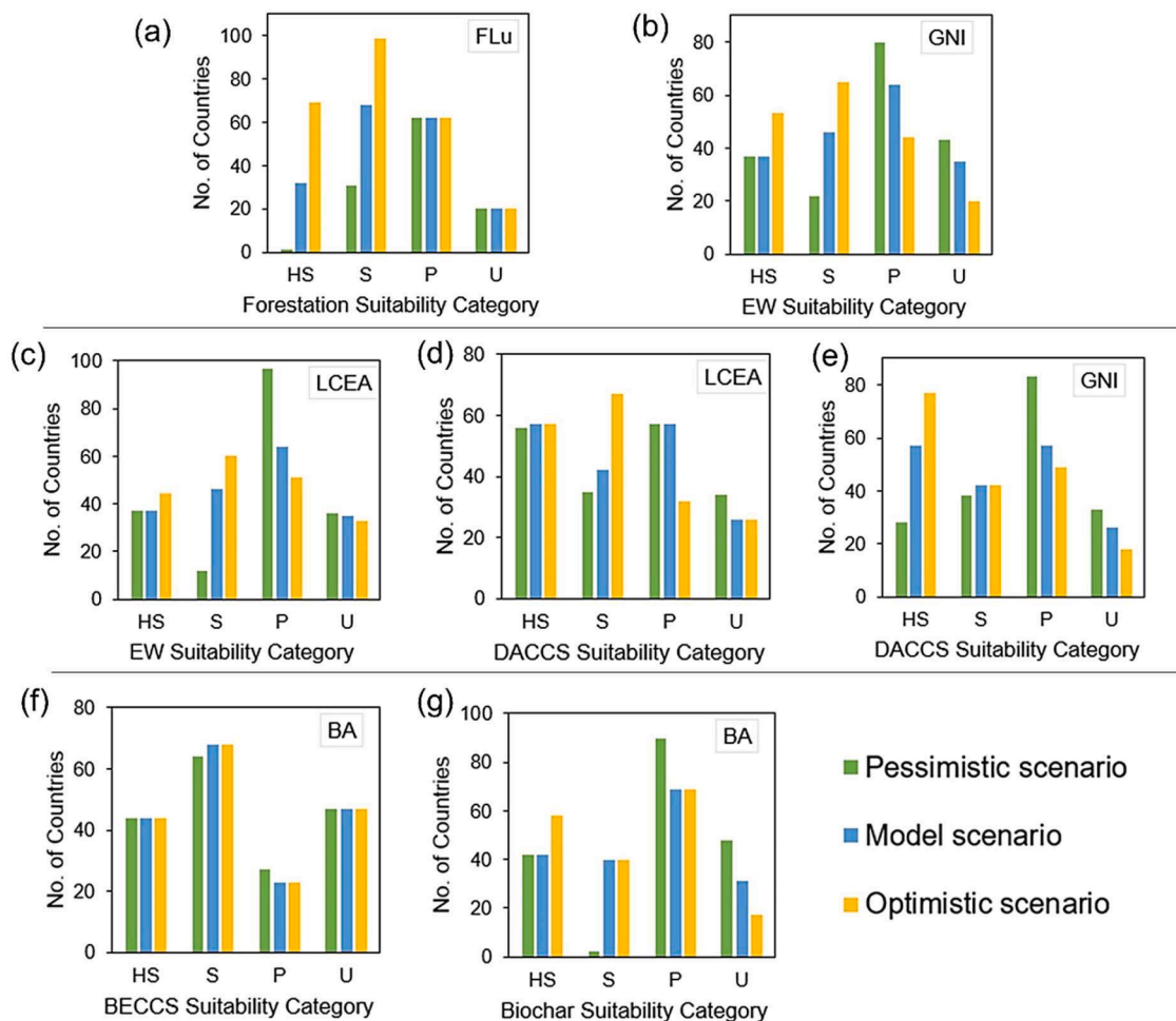
Fig. 5. Impact of resource availability on obtained suitability categorisation (a) FLu on Forestation, (b) GNI on EW, (c) LCEA on EW, (d) LCEA on DACCS, (e) GNI on DACCS, (f) BA on BECCS and (g) BA on biochar.
