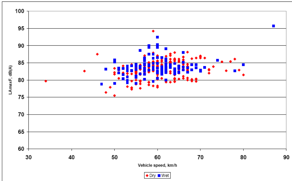
Figure 18 Articulated Trucks L_{max} levels on dry and wet road surface. After Anneck et. al. 2008.
