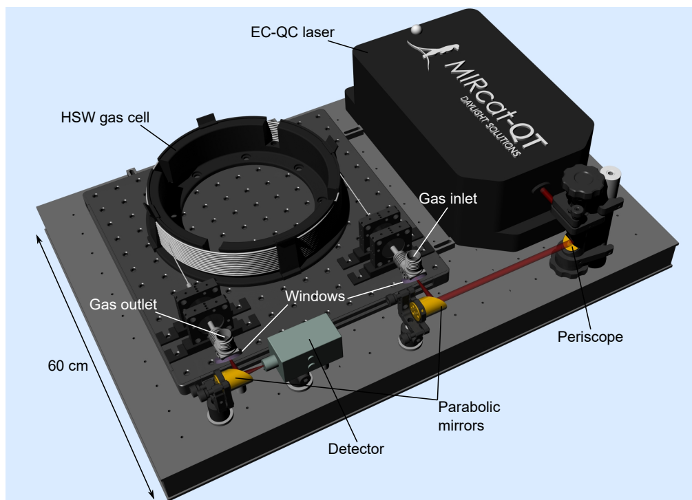
Fig. 1. A 3D diagram showing the layout of components comprising the spectrometer. (STEP files for optomechanics including the small breadboard, lens and mirror mounts, post holders, and periscope mount taken from https://www.thorlabs.com ).
