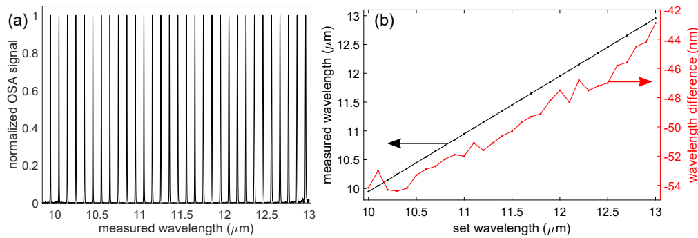
Fig. 2. Plots showing (a) normalized OSA measurements made at 100 nm increments across the 10 – 13 \mu\text{m} range of the tuneable laser, and (b) The variation in measured wavelength vs. the laser set wavelength (left y-axis) and the difference between them (right y-axis).
