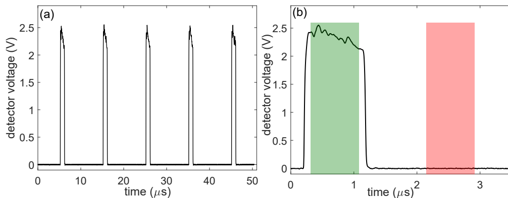
Fig. 4. (a) A plot showing a section of a typical pulse train recorded during a laser sweep. (b) A single pulse with green and red highlighted blocks indicating the approximate region of the on-pulse and off-pulse signal that is averaged and differenced to build up the spectrum.
