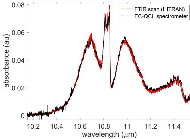
Fig. 7. A plot showing the absorption spectrum of propane in the 10.2 – 11.6 \mu\text{m} region acquired using the external cavity QCL spectrometer. For comparison, the spectrum acquired using an FTIR spectrometer, which is used on the HITRAN database, is also shown [62,63]. The EC-QCL trace (in black) has been processed to the same extent as that in Fig. 6(d).
