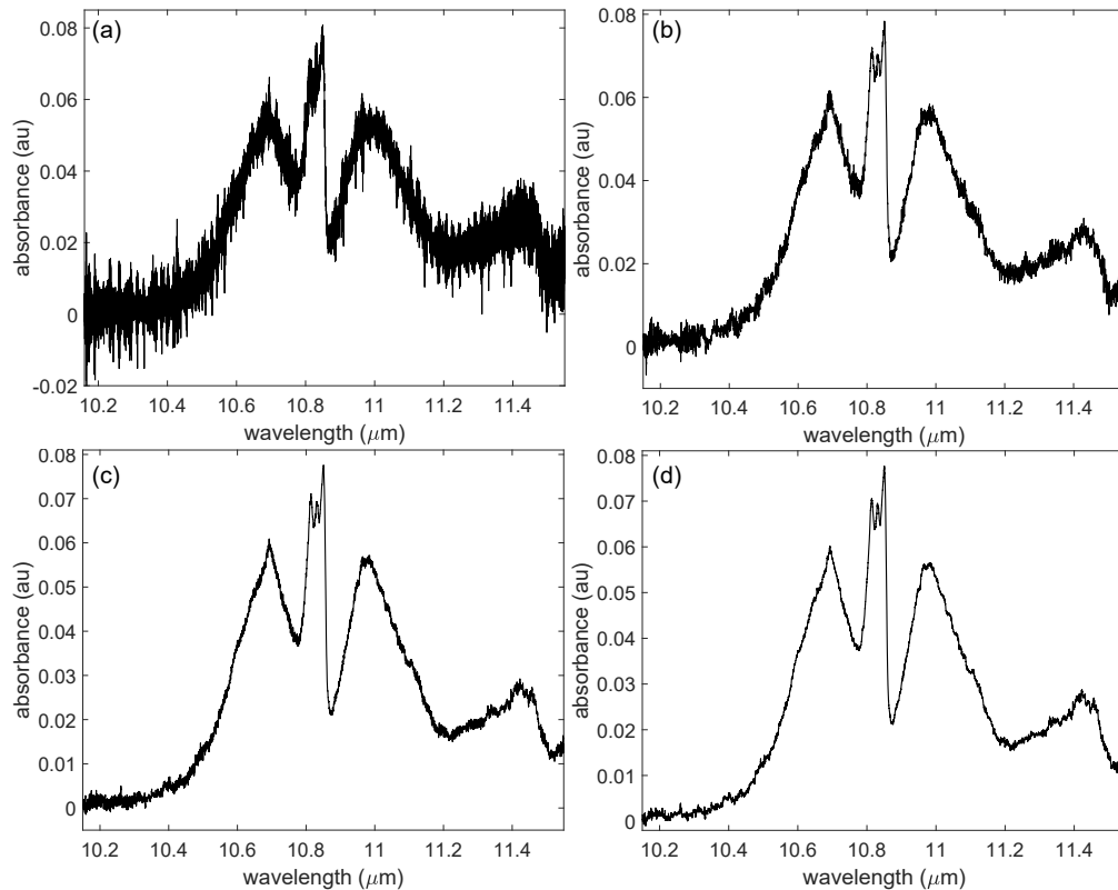
Fig. 6. The processing sequence for normalized absorption spectra acquired in the presence of 1,000 ppm propane: (a) a spectrum obtained using the Beer-Lambert law Eq. (1) on signals obtained with air and propane. (b) after smoothing with a convolution filter. (c) after cumulative averaging, including rejection via baseline comparison, of measurements made over a ~2 minute period. (d) after processing with a Fourier filter.
