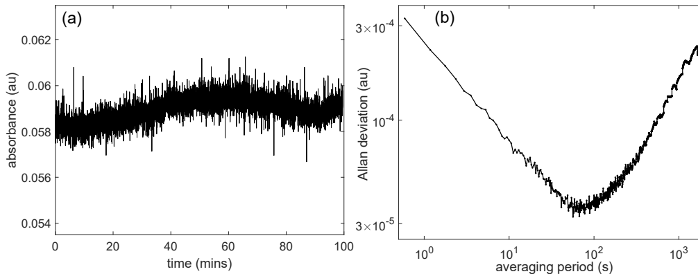
Fig. 10. (a) Time series of absorption data recorded over \sim 100 mins. (b) Allan deviation of that absorption data.
