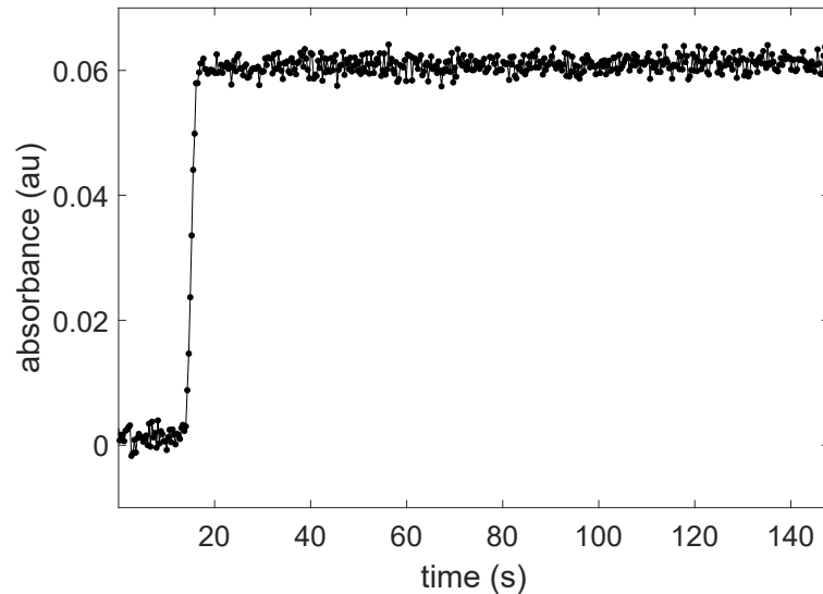
Fig. 8. The variation in absorbance over the course of a measurement. Data was acquired at an increased sweep rate of 50 \mu\text{m s}^{-1} allowing a spectrum acquisition rate of \sim 3 \text{ Hz} , demonstrating the response of the cell. The t_{90} - t_{10} rise time is 1.8 s.
