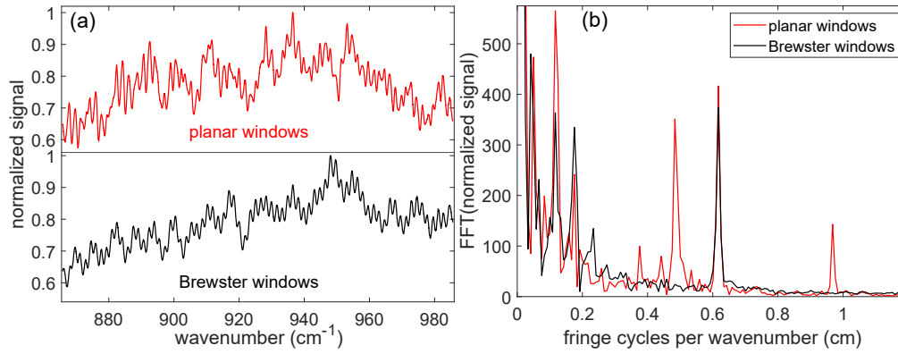
Fig. 5. (a) Raw spectra acquired through hollow waveguide gas cells with planar diamond windows (upper-red) and Brewster aligned diamond windows (lower-black). (b) The FFTs of the signals in (a) with frequencies at 0.48 cm and 0.96 cm associated with the input windows and a frequency at 0.62 cm associated with the output windows.
