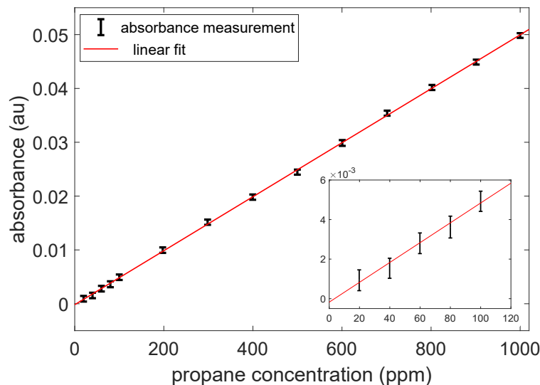
Fig. 9. Absorbance measurements made at a range of propane concentration levels obtained by diluting the flow of propane at 1,000 ppm with zero-grade air. Each point is the mean of values recorded over \sim 2 mins and the error bars are derived from the standard deviation of each measurement step. The linear fit shown has R^2 = 0.9998 . The inset shows the measurements made with the lower flow MFC at concentrations ranging from 20 – 100 ppm more clearly.
