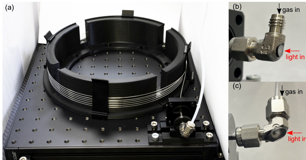
Fig. 3. Photographs showing the construction of the hollow waveguide gas cell: (a) shows the complete cell on the 24 cm diameter, custom designed 3D printed mount, (b) shows a modified Swagelok elbow fitting with a 5 mm diameter normally aligned CVD diamond window embedded, and (c) shows a modified fitting with a 10 mm diameter CVD diamond window aligned at the Brewster angle.
