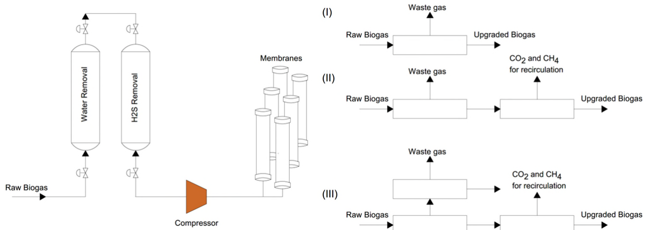
Figure 11. Decarbonisation of biogas using pressure driven dense (gas-gas) membrane separation: (I) single-pass membrane unit, (II) multiple stage membrane units with internal recirculation of permeate, and (III) internal recirculation of retentates[18,46].
