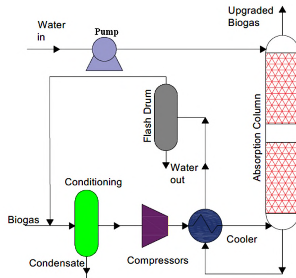
Figure 7. Single-pass water scrubbing for decarbonisation of biogas[7].
